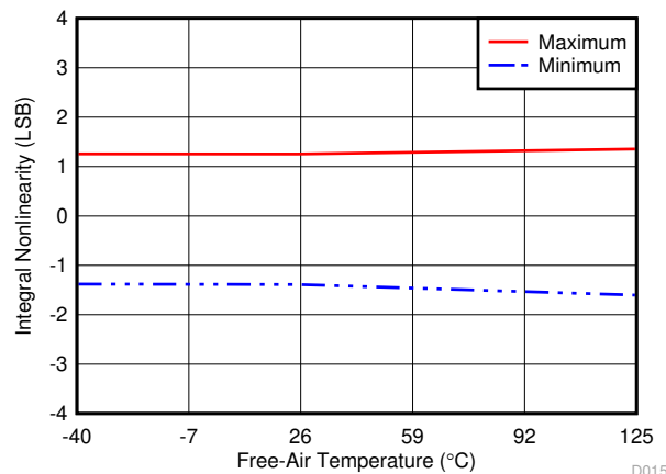
图 6-27. INL vs Temperature (All Unipolar Ranges)
