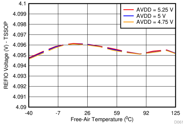
图 7-10. REFIO Voltage Variation Across AVDD and Temperature
