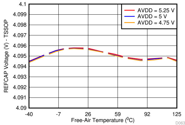
图 7-13. Reference Buffer Output (REFCAP) Variation vs Supply and Temperature
