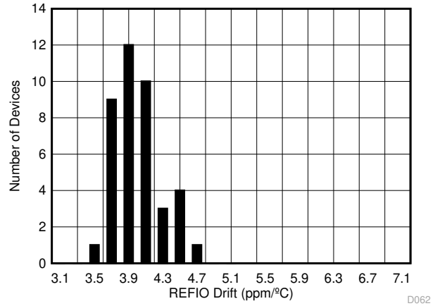
图 7-11. Internal Reference Temperature Drift Histogram
