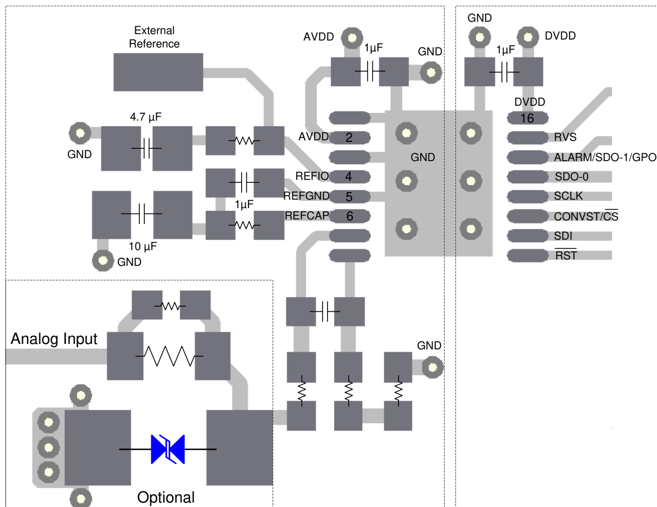
图 10-1. Board Layout for the ADS869x
