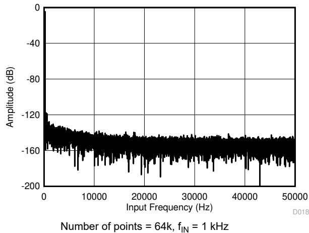
图 6-35. Typical FFT Plot (All Ranges) for the ADS8699
