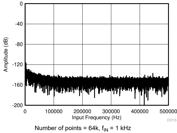
图 6-33. Typical FFT Plot (All Ranges) for the ADS8691
