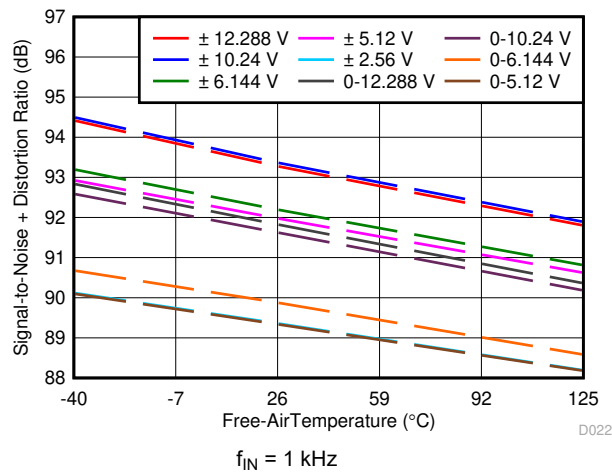
图 6-39. SINAD vs Temperature
