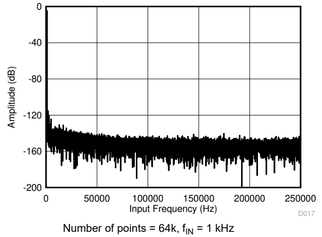
图 6-34. Typical FFT Plot (All Ranges) for the ADS8695
