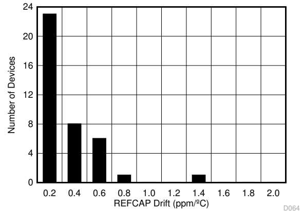
图 7-14. Reference Buffer Temperature Drift Histogram
