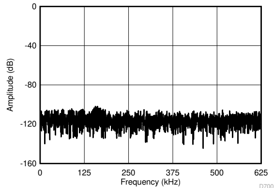
图 8-3. FFT Plot With a DC Common-Mode at 1.25 MSPS
