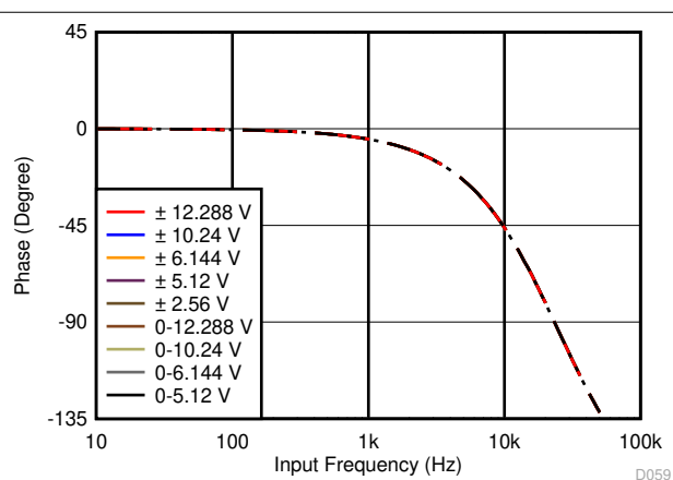
图 7-6. Second-Order LPF Phase Response
