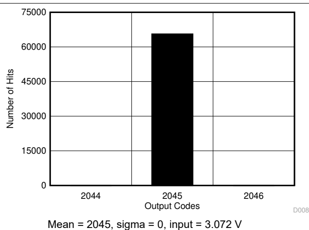
图 6-20. DC Histogram for Mid-Scale Inputs (0 V – 6.144 V)
