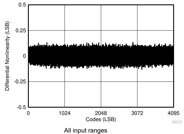
图 6-22. Typical DNL for All Codes
