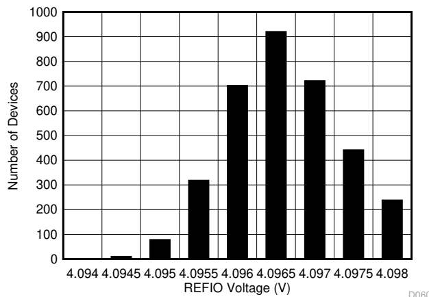
图 7-8. Internal Reference Accuracy Histogram at Room Temperature
