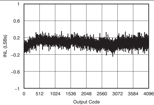
Figure 37. Typical INL
