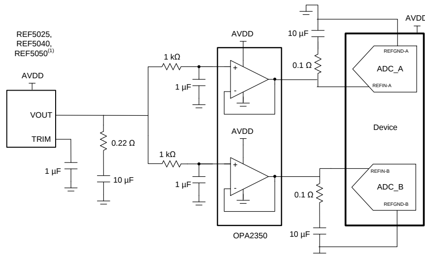
Figure 109. Reference Drive Circuit
