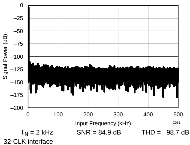
Figure 26. Typical FFT
