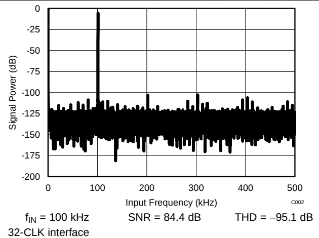
Figure 27. Typical FFT
