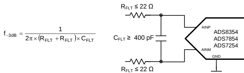
Figure 99. Antialiasing Filter
