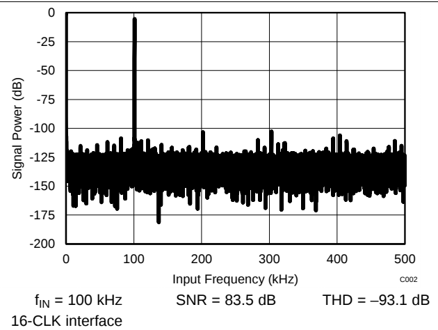
Figure 25. Typical FFT
