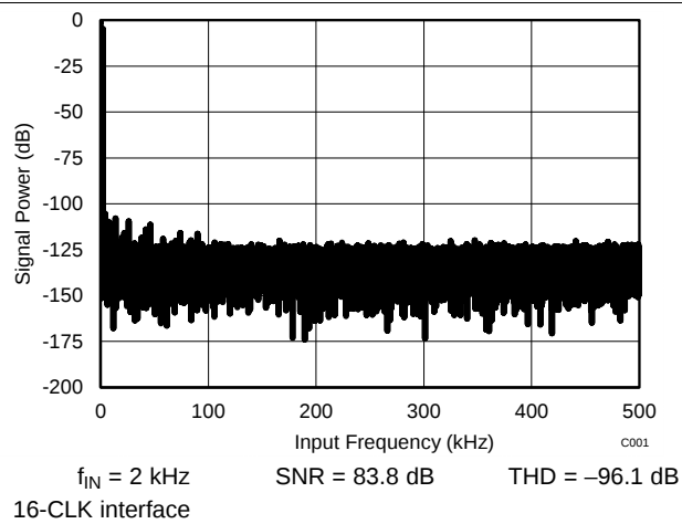
Figure 24. Typical FFT
