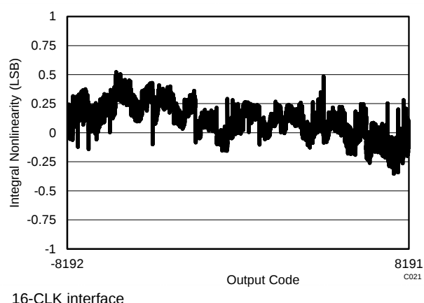
Figure 45. Typical INL
