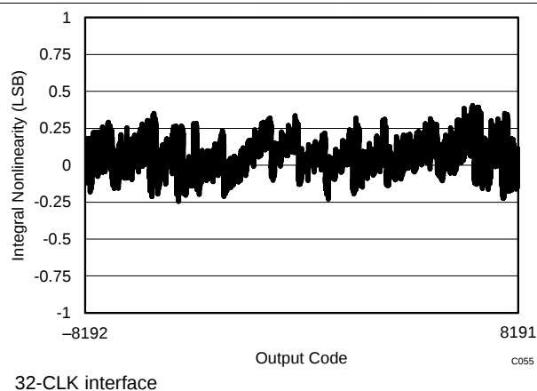
Figure 47. Typical INL
