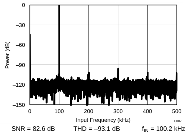
Figure 111. ADS7854 in 32-CLK Interface Mode
