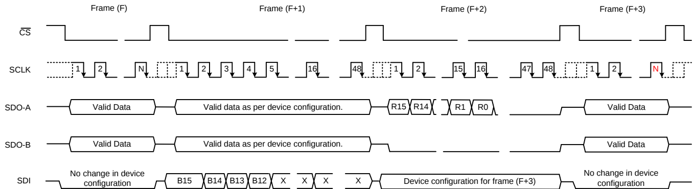
Figure 89. Register Readback Timing
