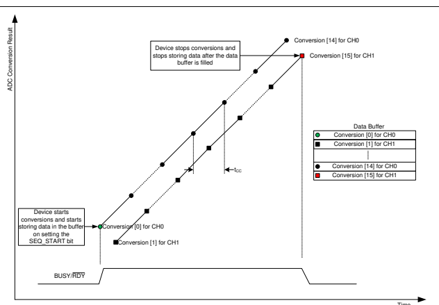
图 7-20. Start Burst With a Dual-Channel Configuration
