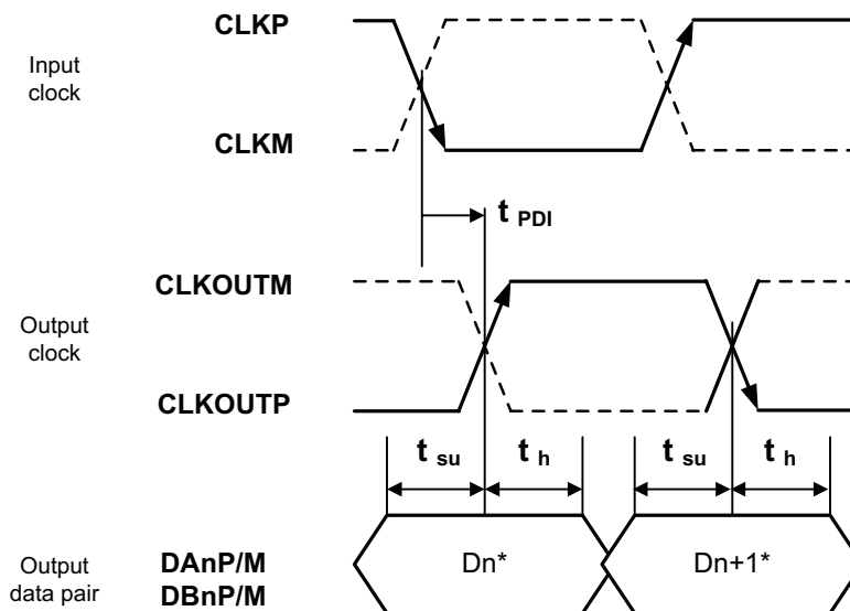
Figure 3. Latency Diagram
