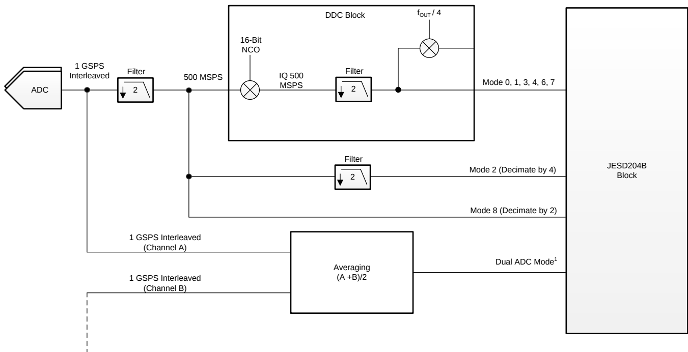
图 49. ADS54J64 Channel Operating Modes
