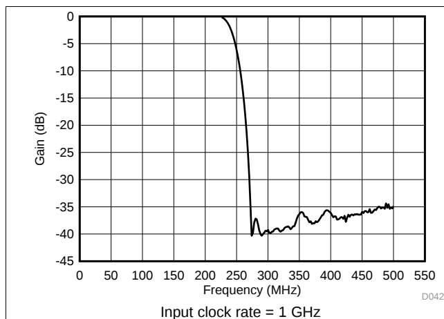
图 50. Decimation Filter Response vs Frequency
