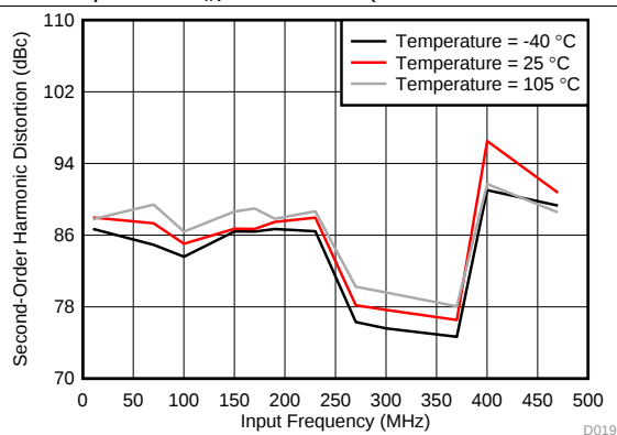
图 20. HD2 vs Input Frequency and Temperature
