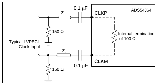
图 47. LVPECL Clock Driving Circuit
