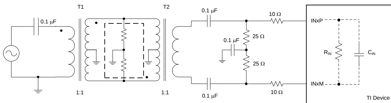
图 46. Analog Input Driving Circuit
