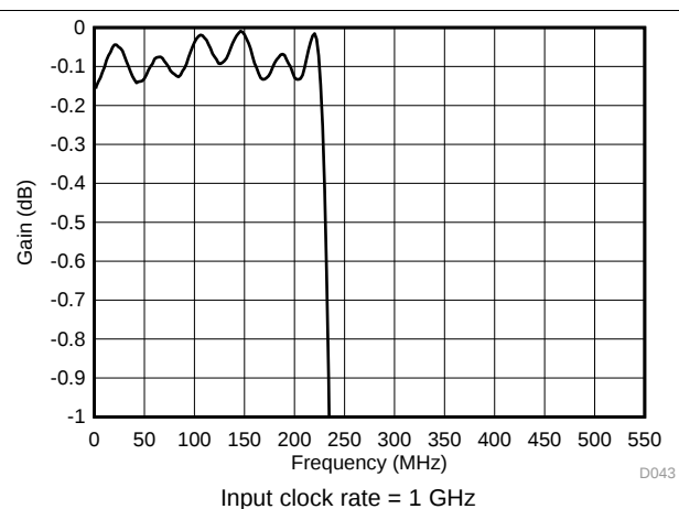
图 51. Decimation Filter Pass-Band Ripple vs Frequency
