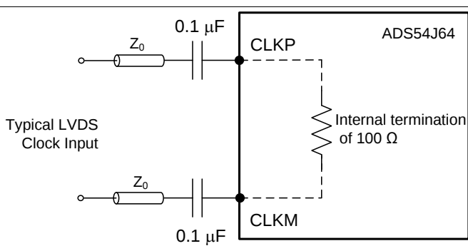
图 48. LVDS Clock Driving Circuit
