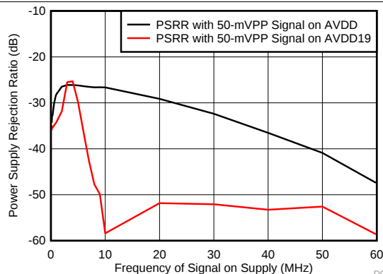
图 32. PSRR vs Power-Supply Noise Frequency
