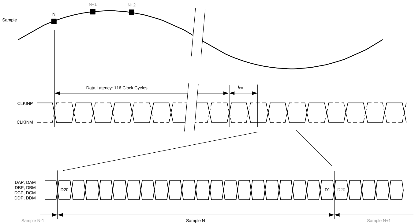
图 1. Latency Timing Diagram in DDC Bypass Mode
