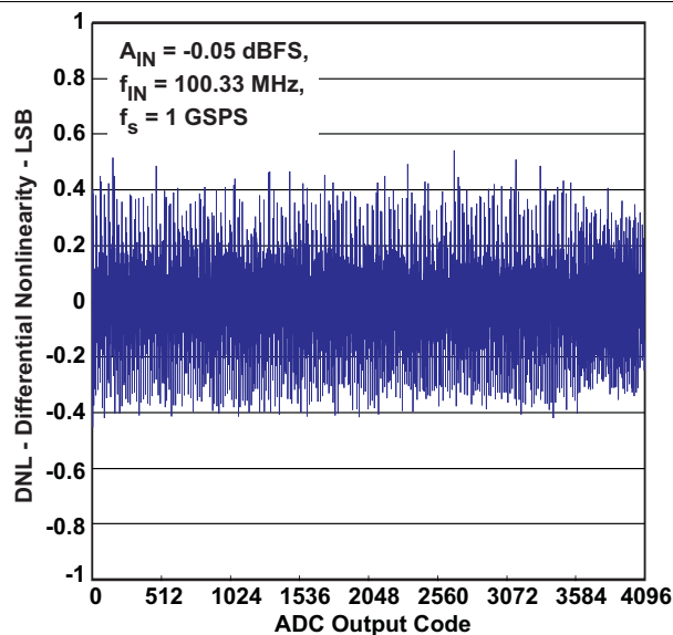
Figure 10. Differential Nonlinearity
