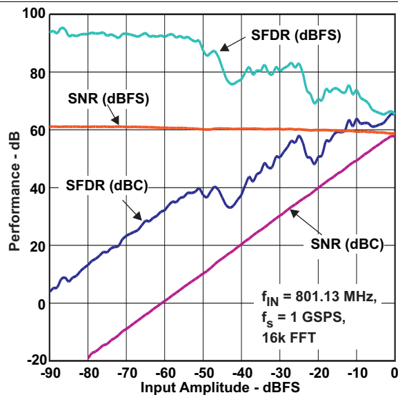
Figure 12. AC Performance vs Input Amplitude (801.13-MHz Input signal)
