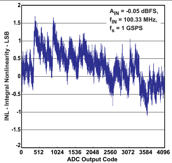
Figure 11. Integral Nonlinearity
