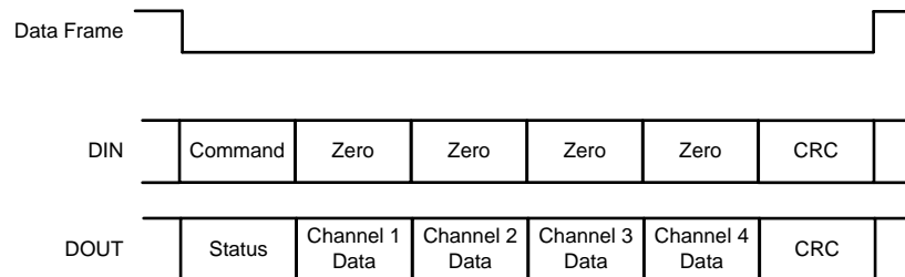
Figure 55. CRC with CRC_MODE = 1
