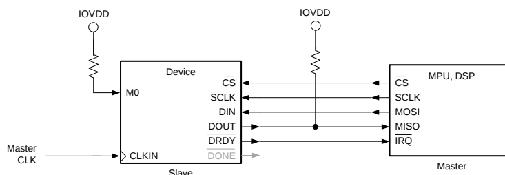
Figure 60. Asynchronous Interrupt Mode Device Connections
