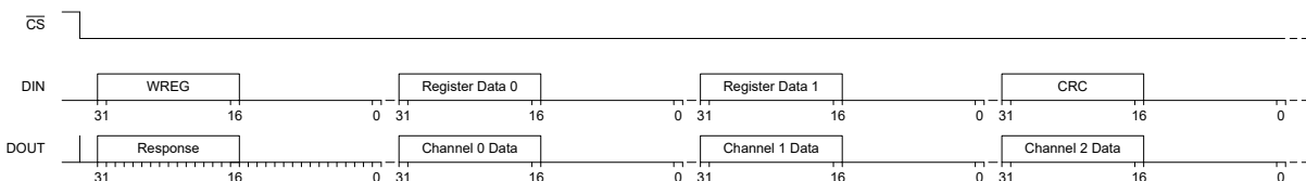
图 8-16. SPI Frame (partial) using 32-bit, zero-padded Word Size
