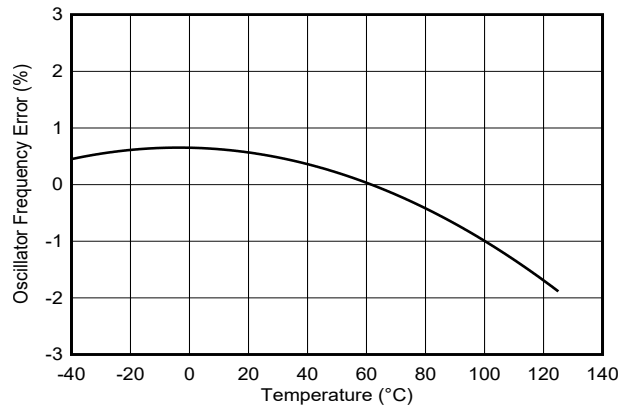
图 6-10. Oscillator Frequency Error vs Temperature
