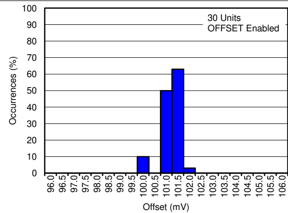
Figure 21. Offset-Voltage Histogram
