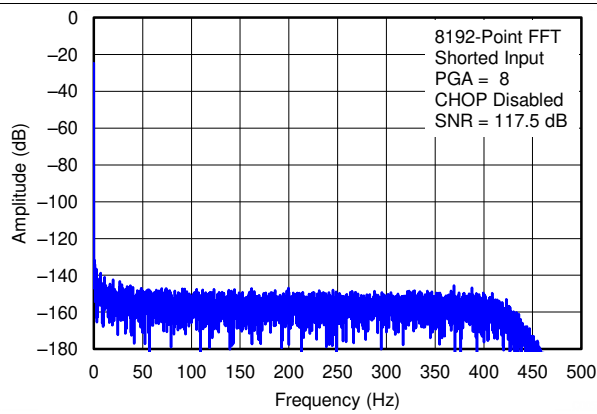
Figure 8. Output Spectrum
