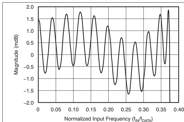
Figure 40. FIR Passband Magnitude Response ( F_{DATA} = 500 Hz)
