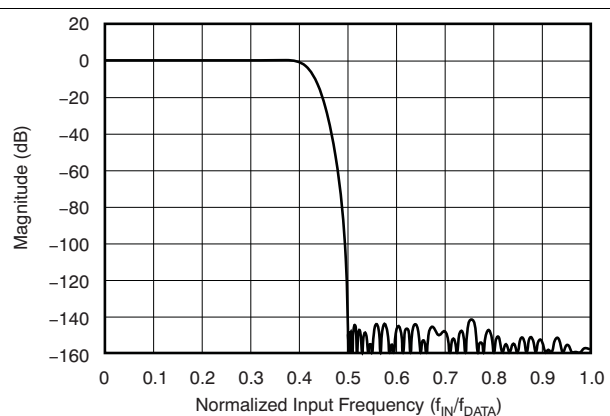
Figure 41. FIR Transition Band Magnitude Response
