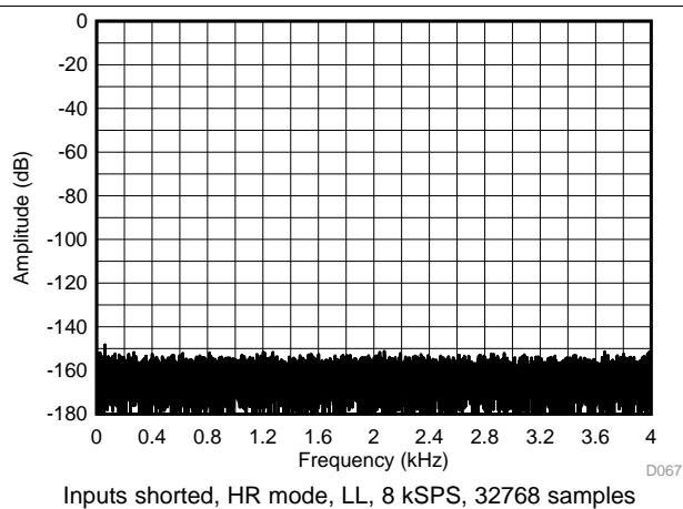
Figure 53. Output Spectrum
