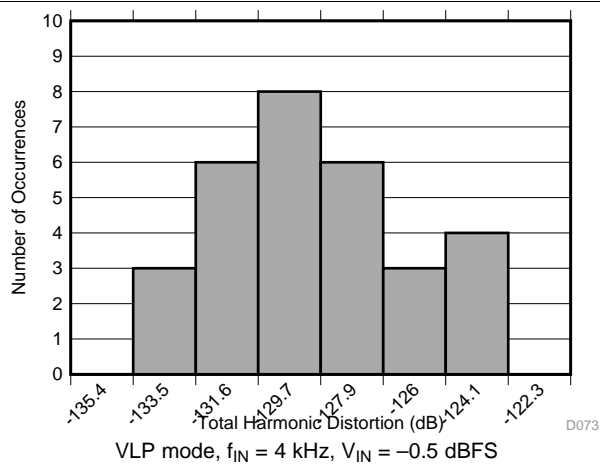
Figure 28. Total Harmonic Distortion Histogram
