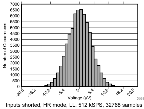
Figure 54. Noise Histogram
