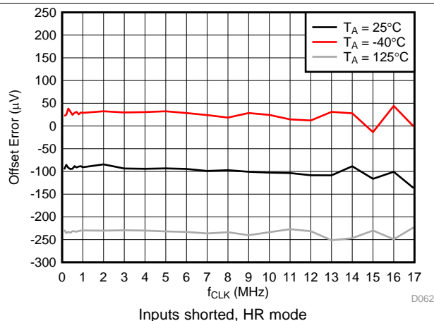
Figure 40. Offset Voltage vs f_{CLK}
