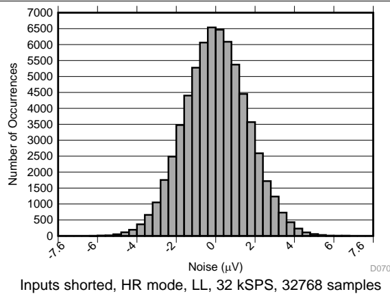
Figure 56. Noise Histogram
