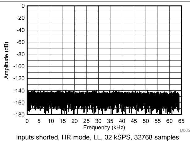
Figure 52. Output Spectrum
