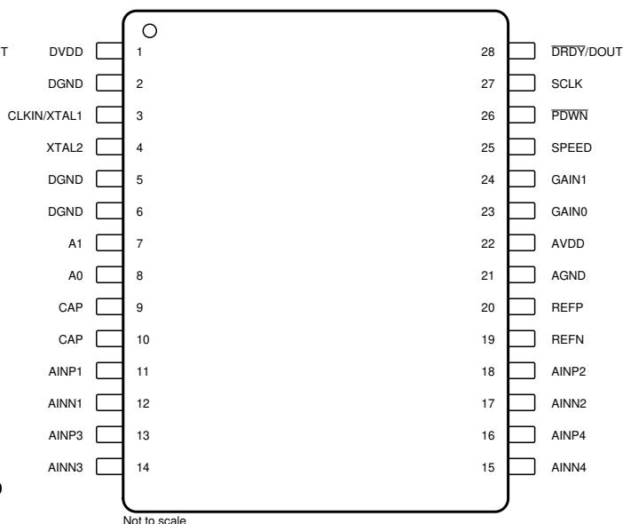
图 4-2. ADS1234 PW Package, 28-Pin TSSOP (Top View)
