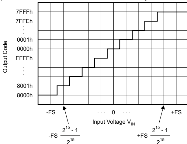
图 7-12. Code Transition Diagram
