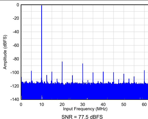
图 6-2. Single Tone FFT at F_{IN} = 10\text{ MHz}
