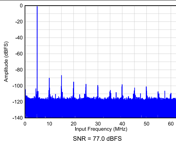
图 6-1. Single Tone FFT at F_{IN} = 5\text{ MHz}
