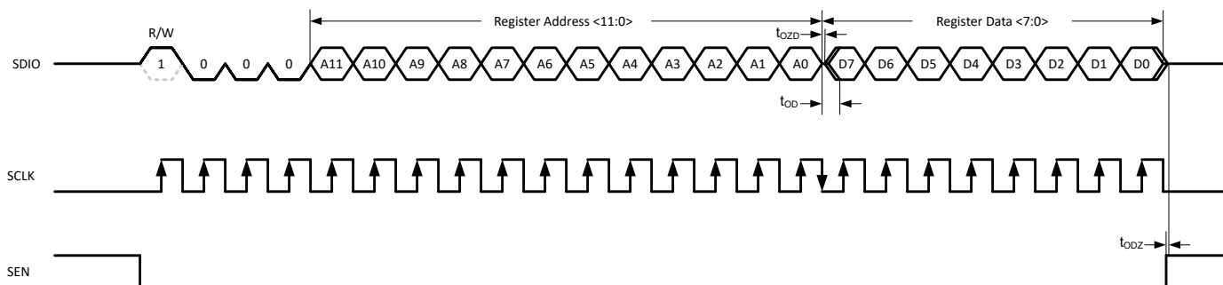
图 8-43. Serial Register Read Timing Diagram
