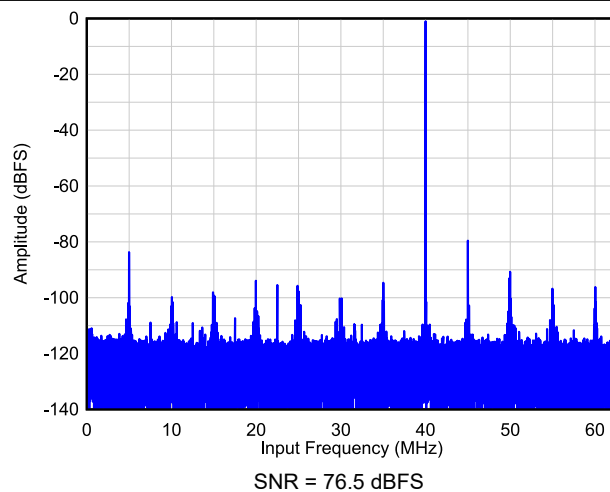
图 6-4. Single Tone FFT at F_{IN} = 40\text{ MHz}
