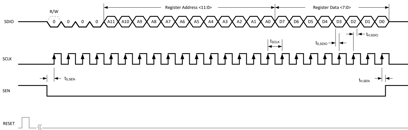
图 8-42. Serial Register Write Timing Diagram
