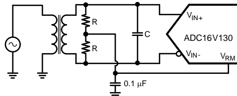
Figure 21. Transformer Drive Circuit for Low Input Frequency
