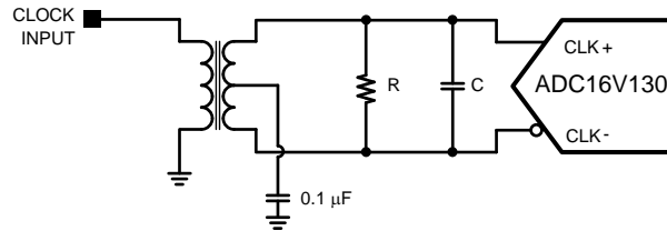
Figure 26. Differential Clocking, Transformer Coupled
