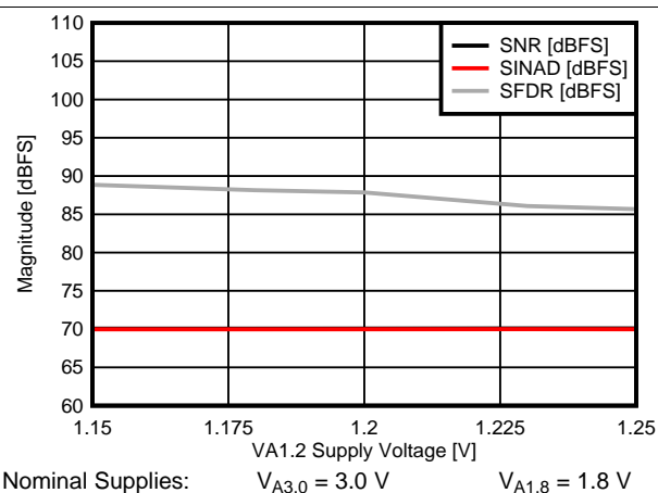
图 18. SNR, SINAD, SFDR vs VA1.2 Supply
