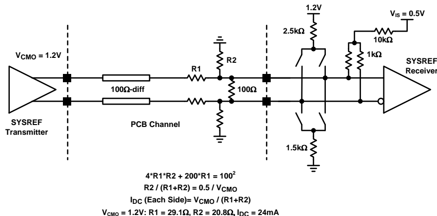
图 51. Example DC Coupling to the SYSREF Input
