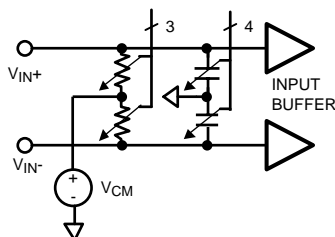
图 32. Simplified Input Differential Balance Correction Circuit
