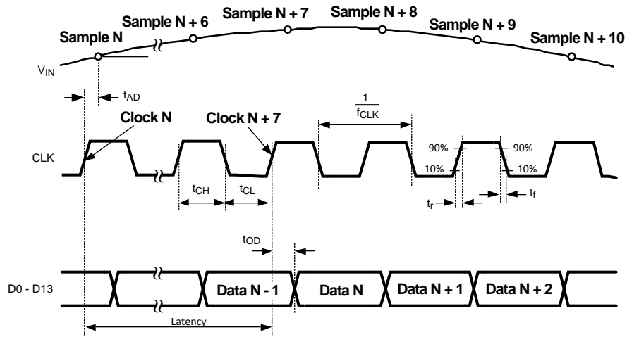
Figure 1. Output Timing
