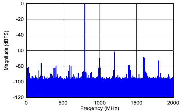
图 5-197. Single-Tone FFT at f_{\text{IN}} = 797\text{MHz} , A_{\text{IN}} = -1\text{dBFS}
