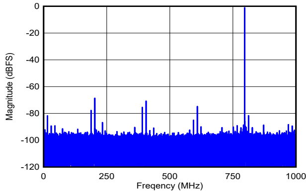
图 5-196. Single-Tone FFT at f_{\text{IN}} = 797\text{MHz} , A_{\text{IN}} = -1\text{dBFS}
