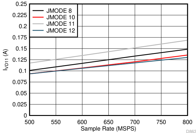
图 7-109. Single Channel, I_{VD11} vs F_S for JMODES 8 - 12
