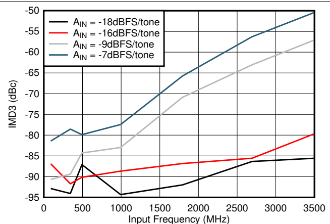
图 7-72. IMD3 vs Input Frequency
