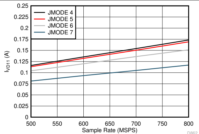
图 7-108. Single Channel, I_{VD11} vs F_S for JMODES 4 - 7
