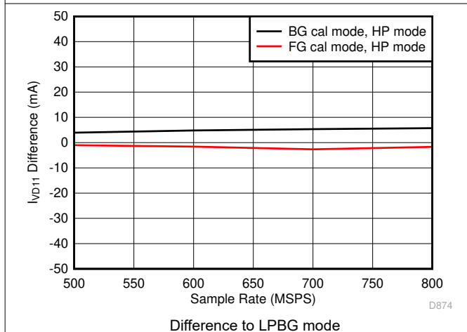
图 5-87. Quad Channel, I_{VD11} vs F_S over Modes
