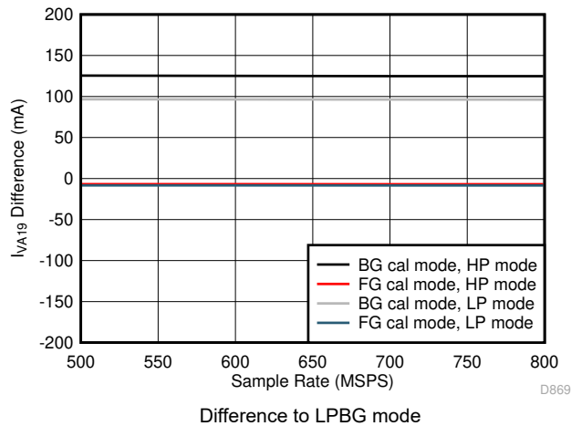
图 7-99. Dual Channel, I_{VA19} vs F_S over Modes
