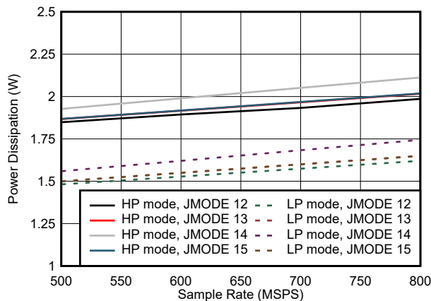
图 7-77. Quad Channel, Power Dissipation vs F_S for JMODES 12 - 15
