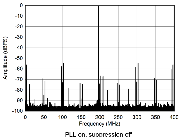
图 7-16. Single Tone FFT at 997 MHz and -1dBFS
