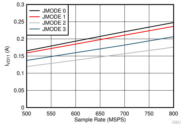
图 7-94. Dual Channel, I_{VD11} vs F_S for JMODES 0 - 3
