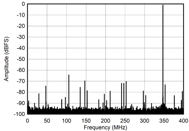
图 7-19. Single Tone FFT at 347 MHz and -1dBFS
