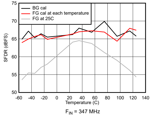
图 7-44. SFDR vs Temperature
