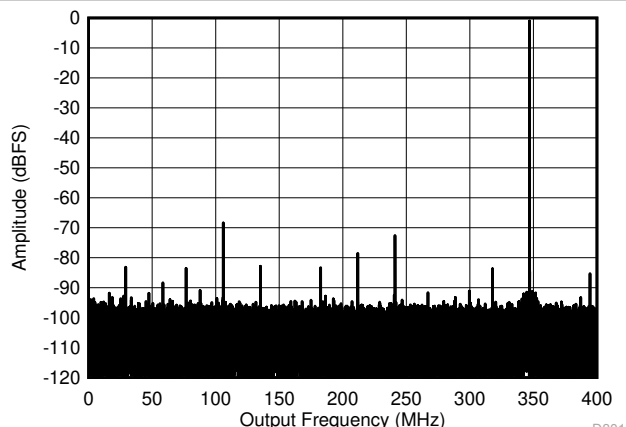
图 7-6. Single Tone FFT at 347 MHz and -1dBFS
