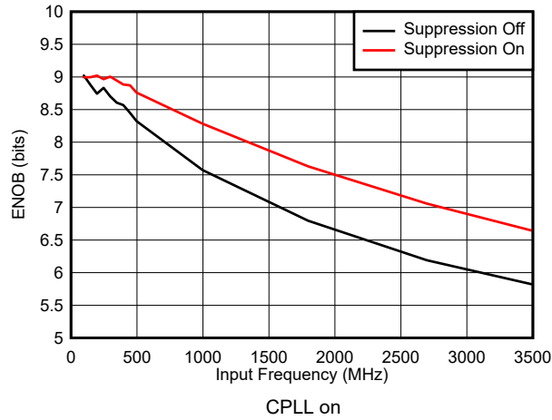
图 7-37. ENOB vs Input Frequency and Suppression
