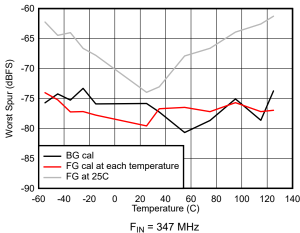
图 7-47. worst non-HD spur vs Temperature
