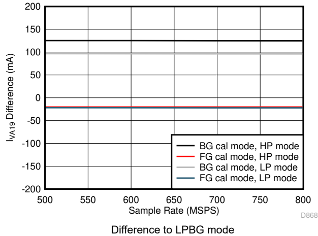
图 7-85. Quad Channel, I_{VA19} vs F_S over Modes
