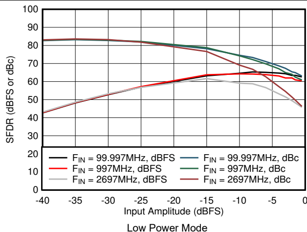
图 7-59. SFDR vs Input Amplitude in Low Power Mode
