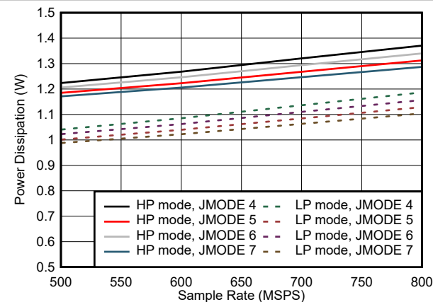
图 7-89. Dual Channel, Power Dissipation vs F_S for JMODES 4 - 7
