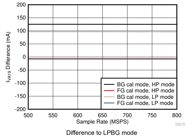
图 7-112. Single Channel, I_{VA19} vs F_S over Modes
