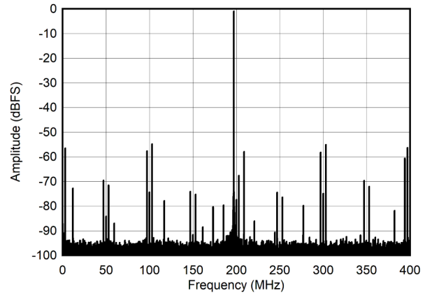
图 7-20. Single Tone FFT at 997 MHz and -1dBFS
