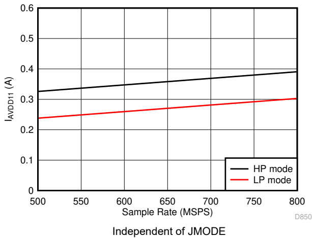
图 7-93. Dual Channel, I_{VA11} vs F_S
