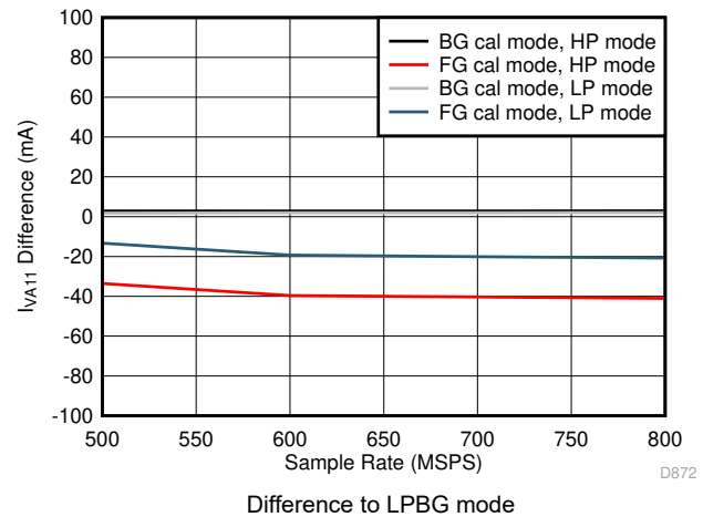
图 7-100. Dual Channel, I_{VA11} vs F_S over Modes
