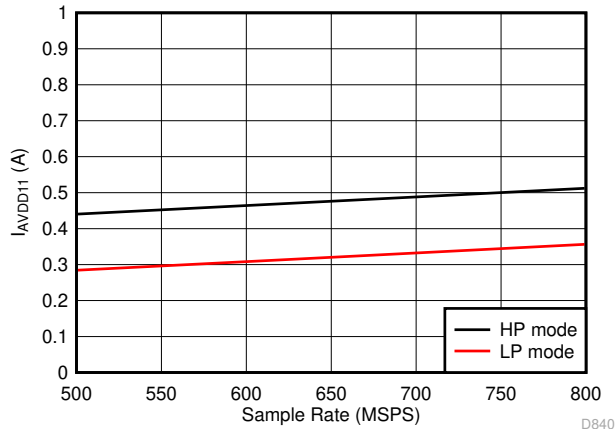
图 7-79. Quad Channel, I_{VA11} vs F_S
