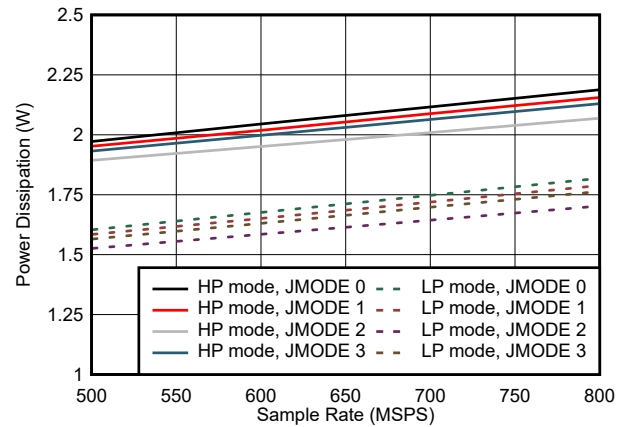
图 7-74. Quad Channel, Power Dissipation vs F_S for JMODES 0 - 3
