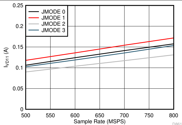
图 7-107. Single Channel, I_{VD11} vs F_S for JMODES 0 - 3
