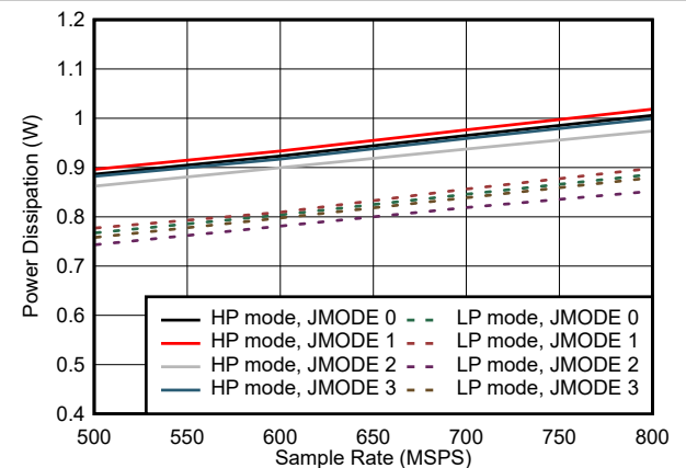
图 7-101. Dual Channel, Power Dissipation vs F_S for JMODES 0 - 3
