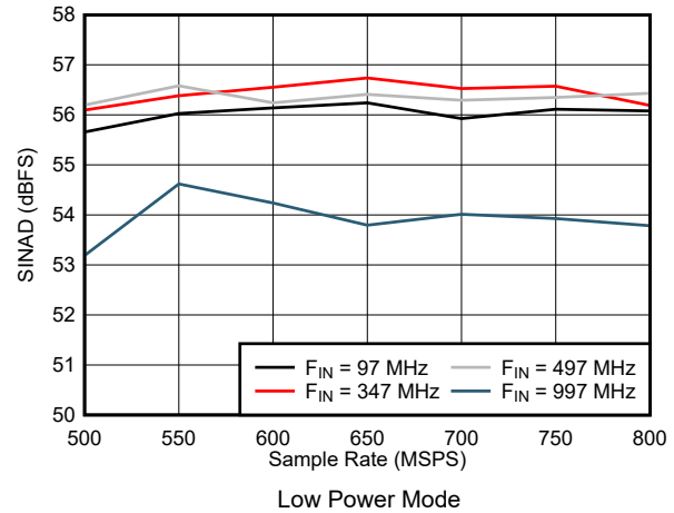
图 7-56. SINAD vs Sample Rate in Low Power Mode
