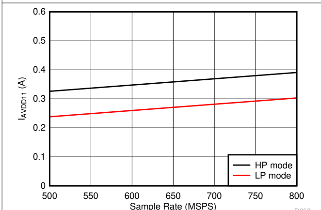
图 5-93. Dual Channel, I_{VA11} vs F_S
