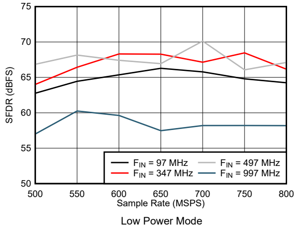
图 7-55. SFDR vs Sample Rate in Low Power Mode
