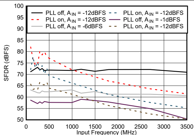
图 7-23. SFDR vs Input Frequency
