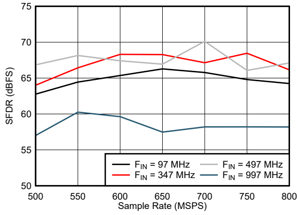
图 5-55. SFDR vs Sample Rate in Low Power Mode
