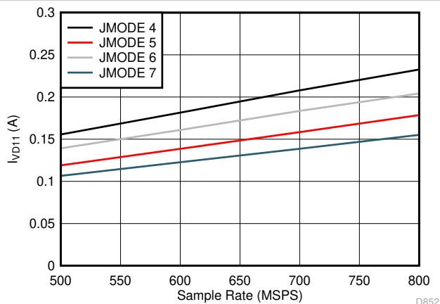
图 7-95. Dual Channel, I_{VD11} vs F_S for JMODES 4 - 7
