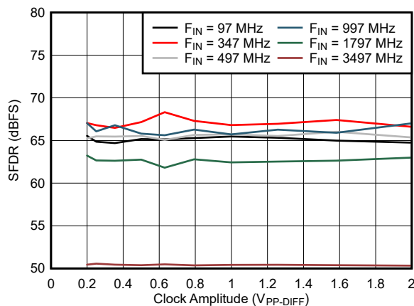
图 7-41. SFDR vs Clock Amplitude
