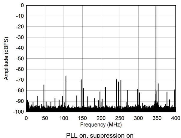
图 7-15. Single Tone FFT at 347 MHz and -1dBFS
