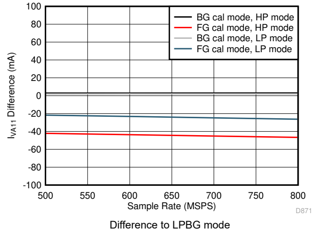
图 7-86. Quad Channel, I_{VA11} vs F_S over Modes
