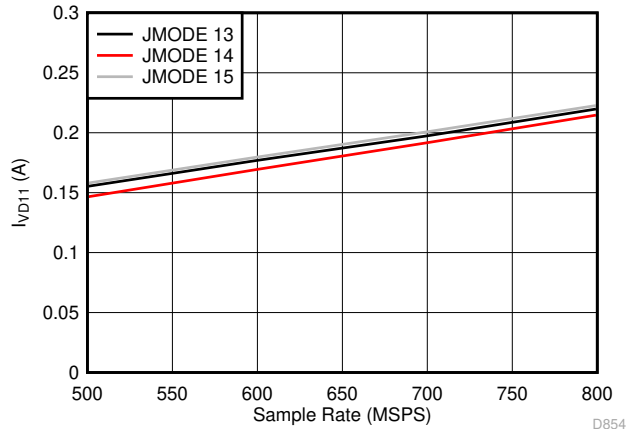
图 7-97. Dual Channel, I_{VD11} vs F_S for JMODES 13 - 15
