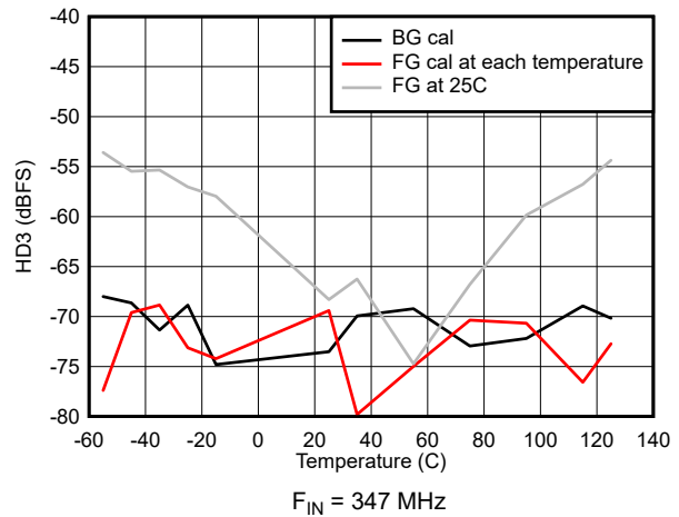
图 7-46. HD3 vs Temperature
