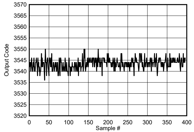
图 7-116. Background Calibration Core Transition (voltage offset)
