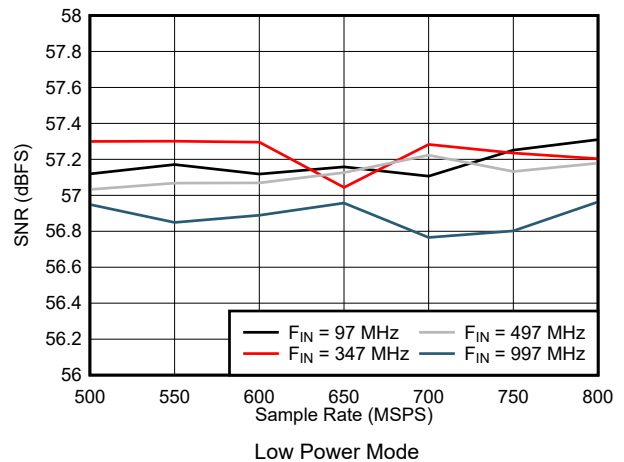
图 7-54. SNR vs Sample Rate in Low Power Mode
