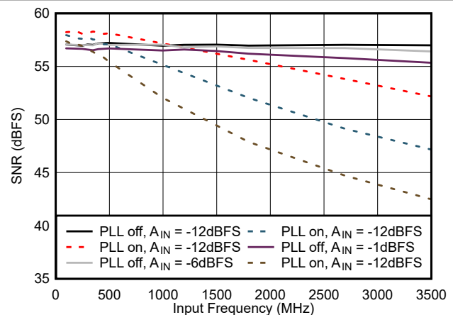
图 7-22. SNR vs Input Frequency
