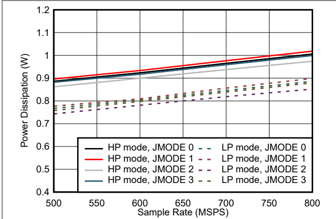
图 5-101. Dual Channel, Power Dissipation vs F_S for JMODES 0 - 3
