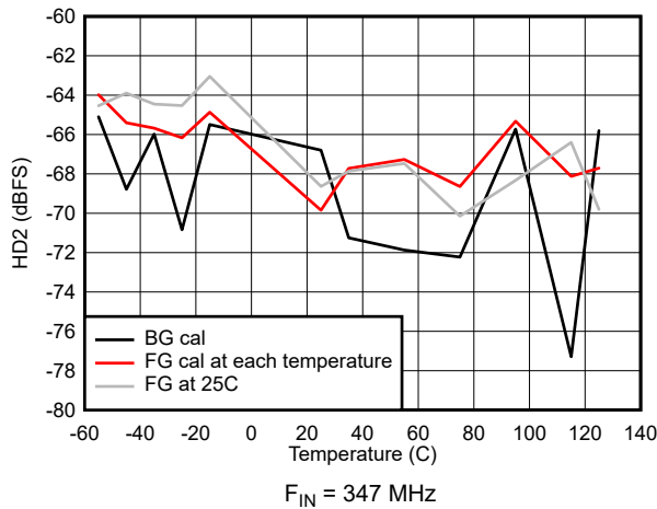
图 7-45. HD2 vs Temperature
