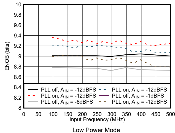
图 7-53. ENOB vs Input Frequency in Low Power Mode
