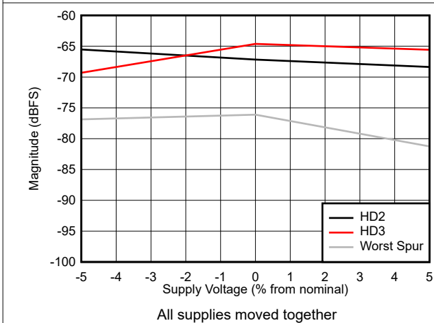
图 5-39. HD2, HD3 and worst non-HD vs Supply Voltage
