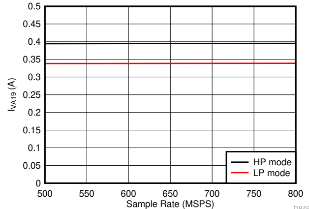
图 7-92. Dual Channel, I_{VA19} vs F_S
