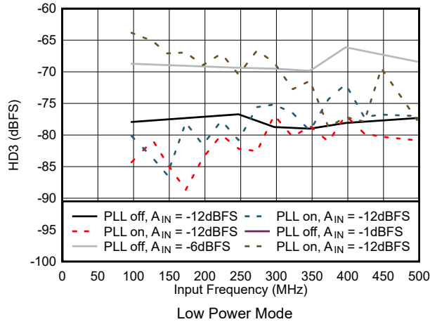
图 7-51. HD3 vs Input Frequency in Low Power Mode
