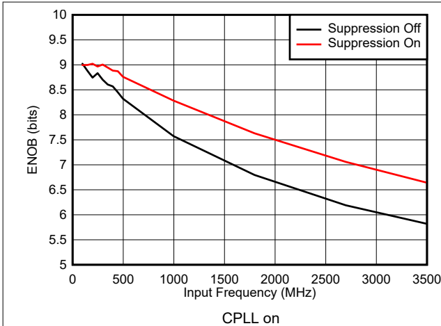
图 5-37. ENOB vs Input Frequency and Suppression
