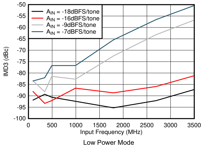
图 7-73. IMD3 vs Input Frequency in Low Power Mode
