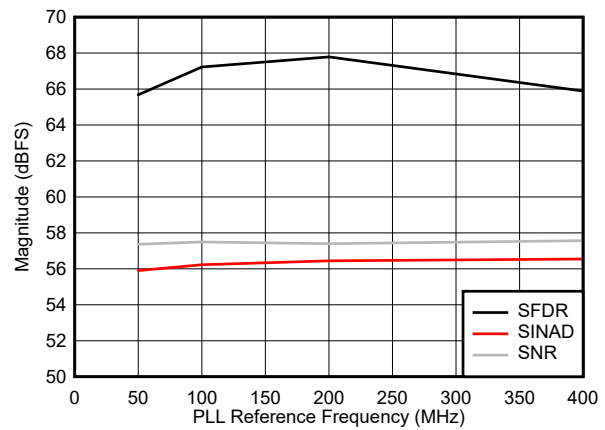
图 7-42. SNR, SFDR and SINAD vs Reference Frequency with PLL on
