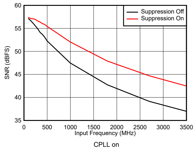
图 7-34. SNR vs Input Frequency and Suppression
