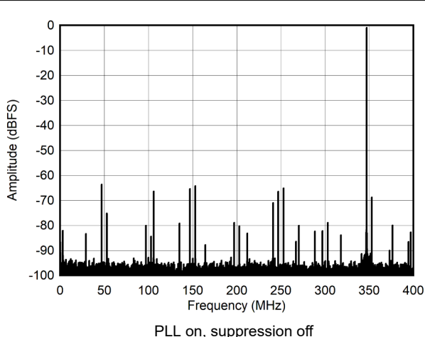
图 7-14. Single Tone FFT at 347 MHz and -1dBFS
