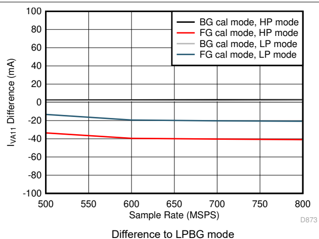
图 7-113. Single Channel, I_{VA11} vs F_S over Modes
