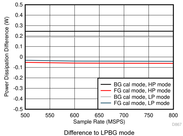
图 7-111. Single Channel, Power Dissipation vs F_S over Modes
