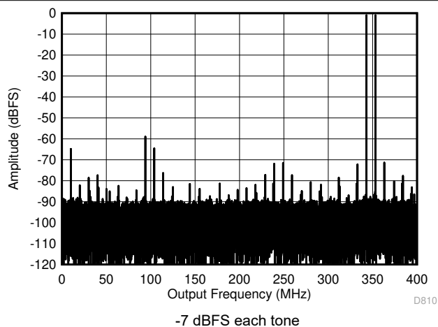
图 7-69. Two Tone FFT at 347 MHz in Low Power Mode
