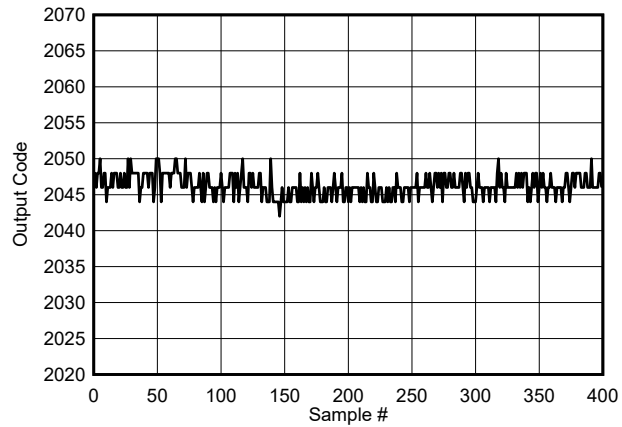
图 7-115. Background Calibration Core Transition (midscale)
