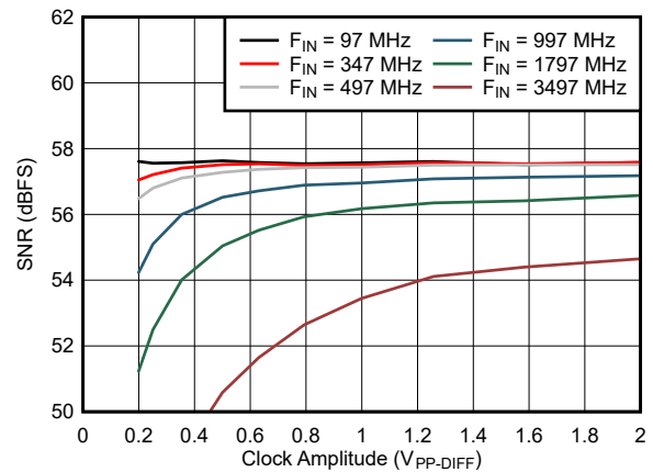
图 7-40. SNR vs Clock Amplitude
