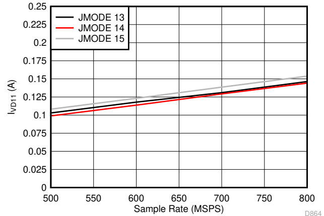
图 7-110. Single Channel, I_{VD11} vs F_S for JMODES 13 - 15
