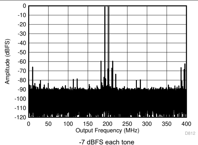
图 7-70. Two Tone FFT at 1798 MHz in Low Power Mode
