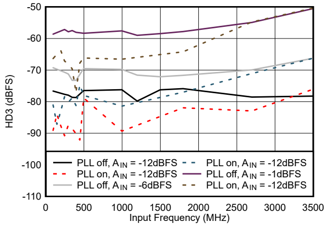
图 7-25. HD3 vs Input Frequency
