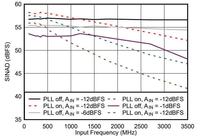
图 7-26. SINAD vs Input Frequency
