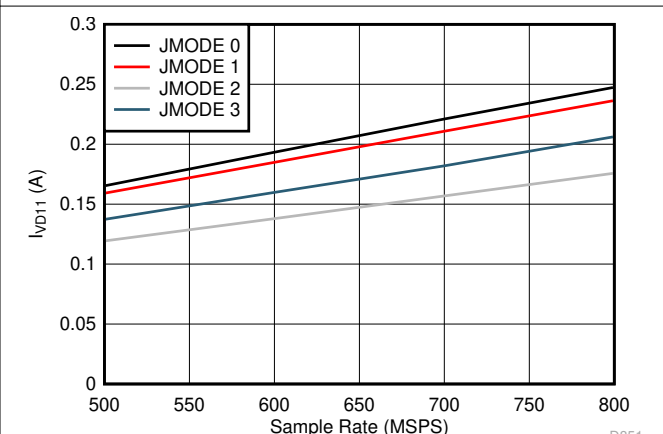
图 5-94. Dual Channel, I_{VD11} vs F_S for JMODES 0 - 3
