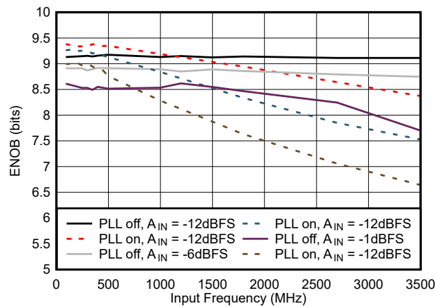
图 7-27. ENOB vs Input Frequency
