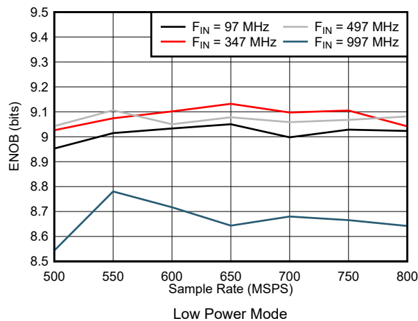
图 7-57. ENOB vs Sample Rate in Low Power Mode
