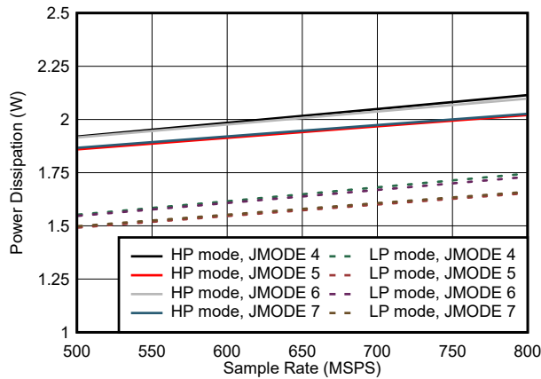
图 7-75. Quad Channel, Power Dissipation vs F_S for JMODES 4 - 7
