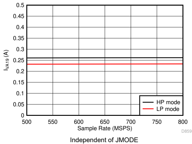
图 7-105. Single Channel, I_{VA19} vs F_S
