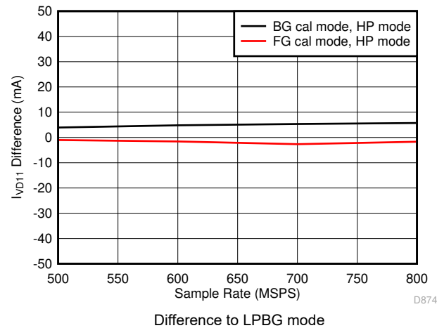
图 7-87. Quad Channel, I_{VD11} vs F_S over Modes
