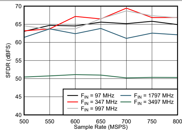
图 7-29. SFDR vs Sample Rate
