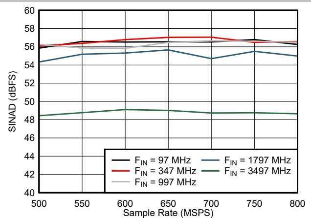
图 7-30. SINAD vs Sample Rate
