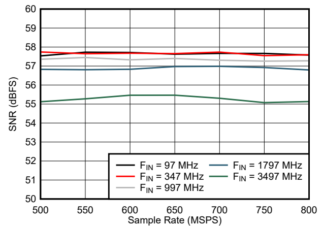
图 7-28. SNR vs Sample Rate
