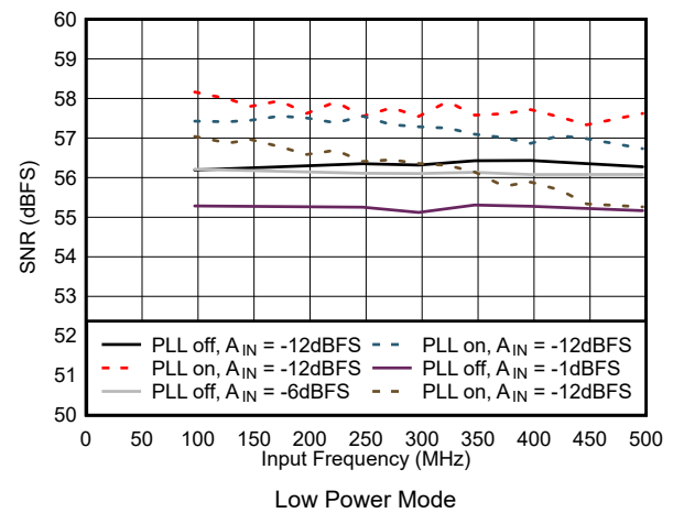
图 7-48. SNR vs Input Frequency in Low Power Mode
