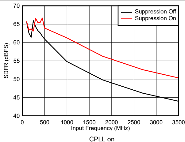
图 7-35. SFDR vs Input Frequency and Suppression
