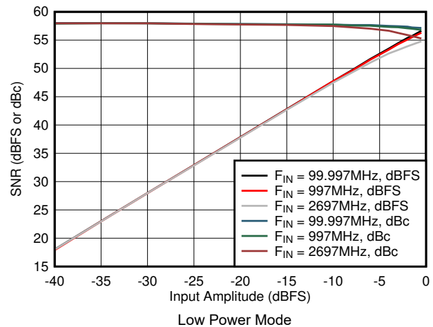
图 7-58. SNR vs Input Amplitude in Low Power Mode
