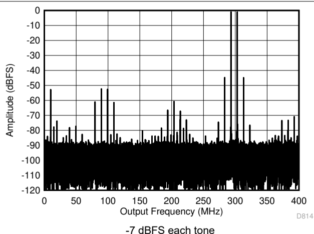
图 7-71. Two Tone FFT at 3498 MHz in Low Power Mode
