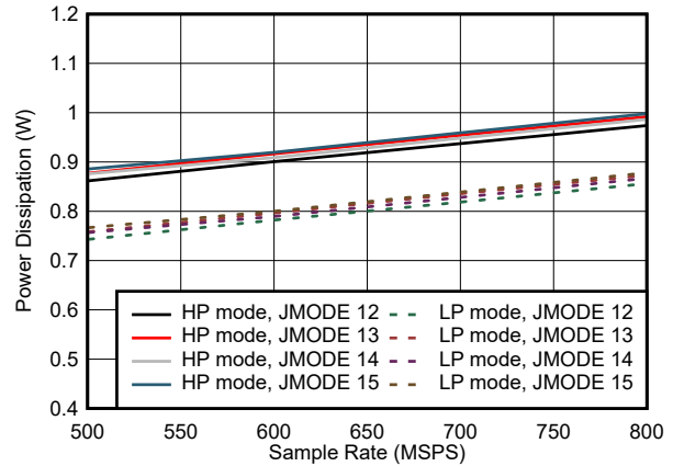
图 7-104. Single Channel, Power Dissipation vs F_S for JMODES 12 - 15
