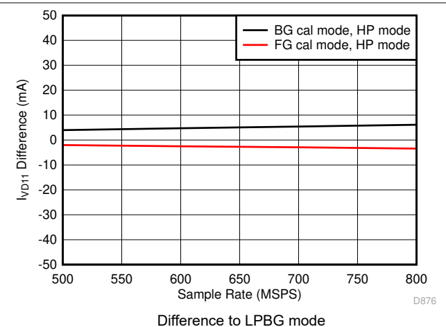
图 7-114. Single Channel, I_{VD11} vs F_S over Modes
