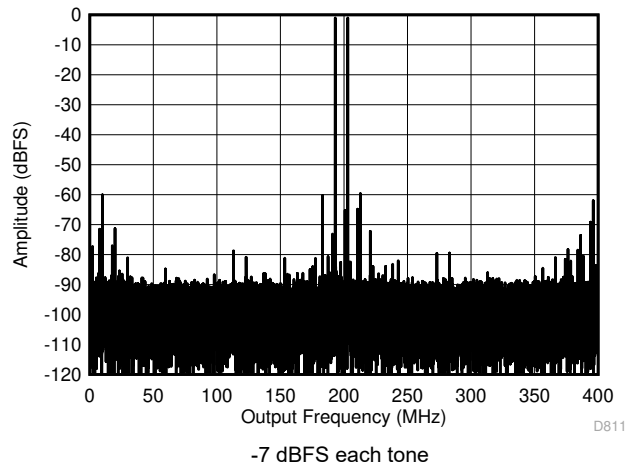
图 7-67. Two Tone FFT at 1798 MHz
