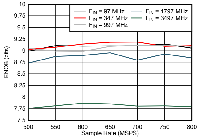
图 7-31. ENOB vs Sample Rate
