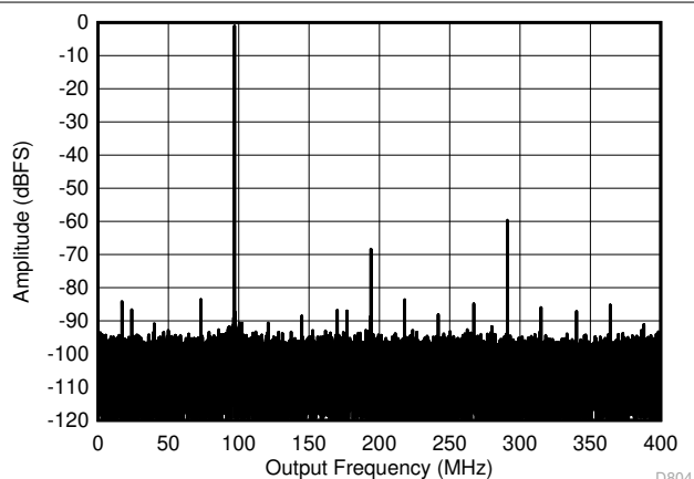
图 7-11. Single Tone FFT at 897 MHz and -1dBFS Low Power Mode
