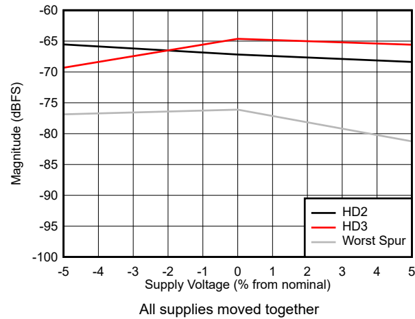
图 7-39. HD2, HD3 and worst non-HD vs Supply Voltage
