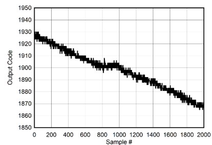
图 7-116. Background Calibration Core Transition (voltage offset)
