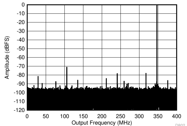
图 7-10. Single Tone FFT at 347 MHz and -1dBFS Low Power Mode
