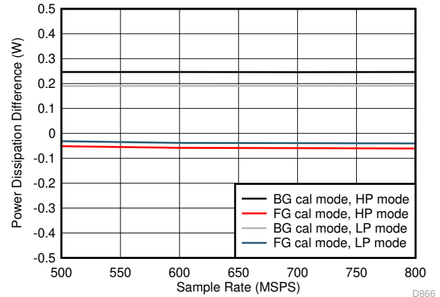
图 7-98. Dual Channel, Power Dissipation vs F_S over Modes
