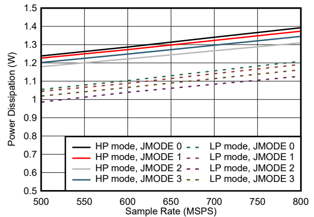
图 7-88. Dual Channel, Power Dissipation vs F_S for JMODES 0 - 3
