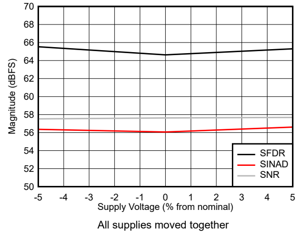
图 7-38. SNR, SFDR and SINAD vs Supply Voltage
