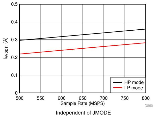
图 7-106. Single Channel, I_{VA11} vs F_S
