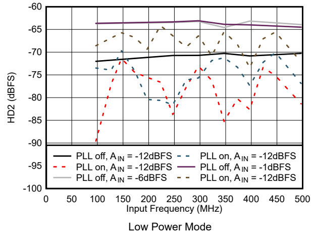
图 7-50. HD2 vs Input Frequency in Low Power Mode
