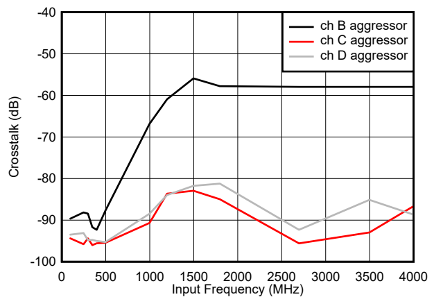
图 7-4. Crosstalk vs Input Frequency, Channel A victim
