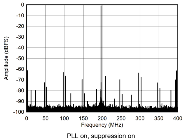
图 7-17. Single Tone FFT at 997 MHz and -1dBFS
