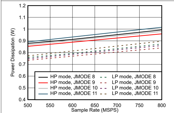
图 5-103. Single Channel, Power Dissipation vs F_S for JMODES 8 - 11
