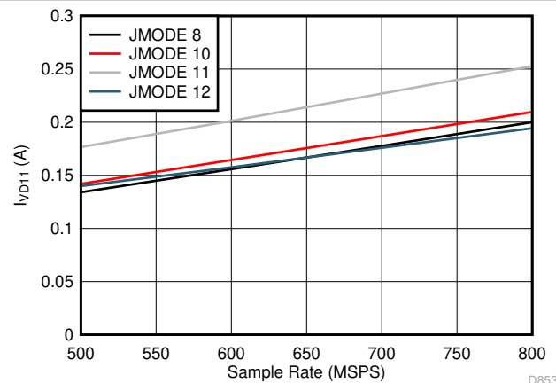
图 7-96. Dual Channel, I_{VD11} vs F_S for JMODES 8 - 12
