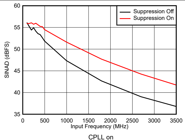
图 7-36. SINAD vs Input Frequency and Suppression
