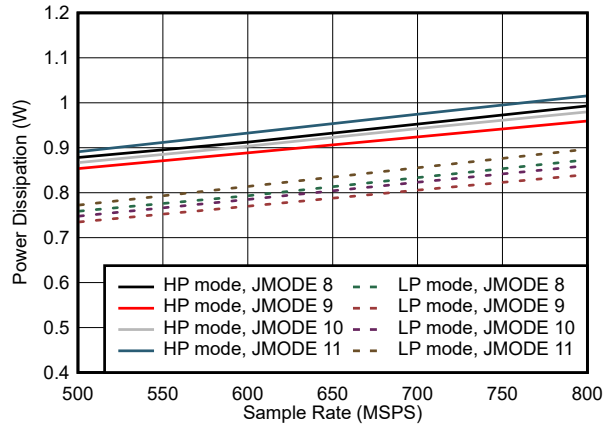
图 7-103. Single Channel, Power Dissipation vs F_S for JMODES 8 - 11
