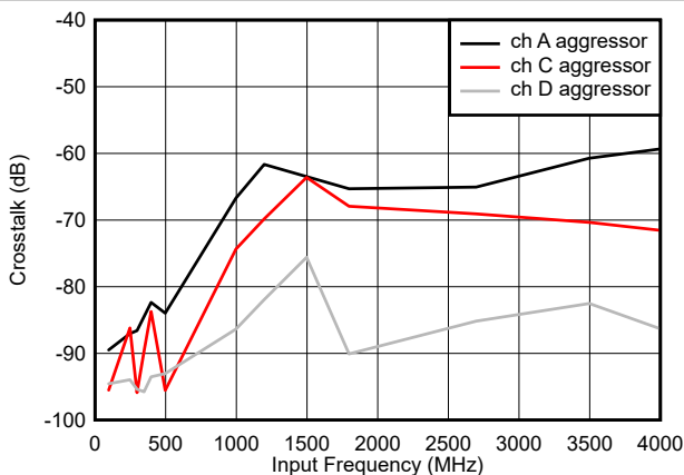
图 7-5. Crosstalk vs Input Frequency, Channel B victim
