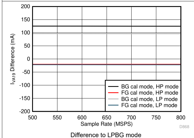
图 5-85. Quad Channel, I_{VA19} vs F_S over Modes
