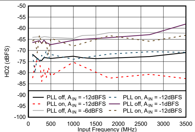
图 7-24. HD2 vs Input Frequency
