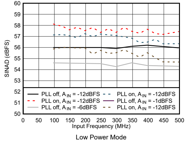
图 7-52. SINAD vs Input Frequency in Low Power Mode
