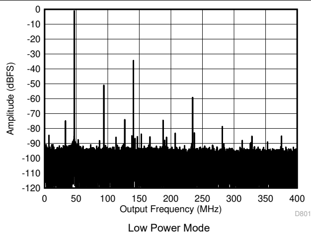
图 7-13. Single Tone FFT at 3247 MHz and -1dBFS
