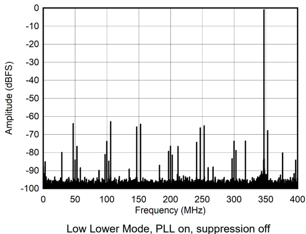
图 7-18. Single Tone FFT at 347 MHz and -1dBFS
