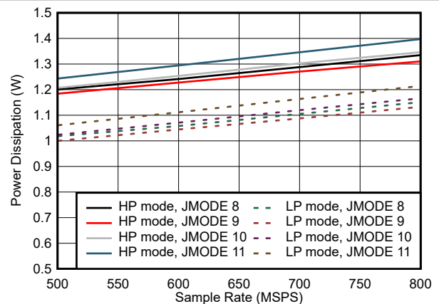
图 7-90. Dual Channel, Power Dissipation vs F_S for JMODES 8 - 11
