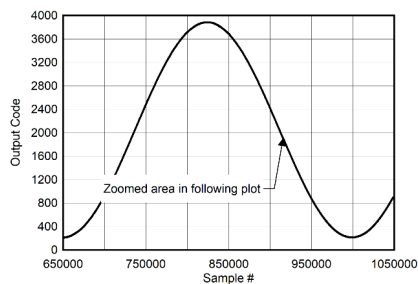
图 7-115. Background Calibration Core Transition (midscale)
