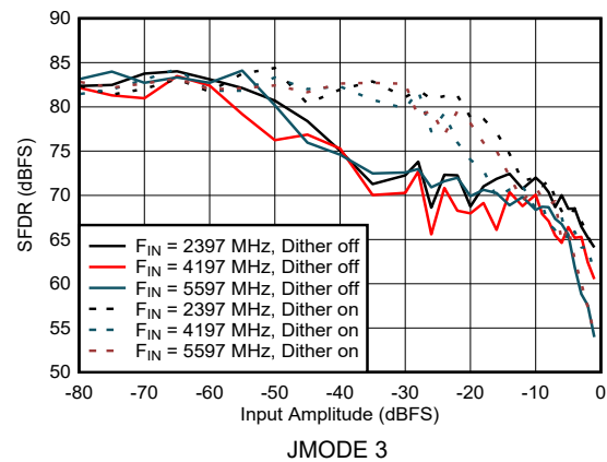
图 6-40. Dual Channel Mode: SFDR vs Input Amplitude
