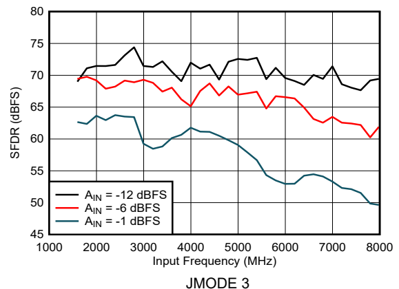
图 6-34. Dual Channel Mode: SFDR vs Input Frequency
