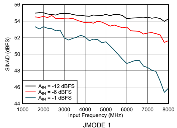
图 6-10. DES Mode: SINAD vs Input Frequency
