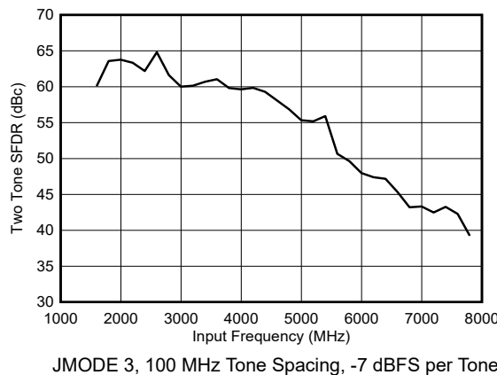
图 6-45. Dual Channel Mode: Two Tone SFDR vs Input Frequency
