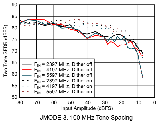
图 6-47. Dual Channel Mode: Two Tone SFDR vs Input Amplitude
