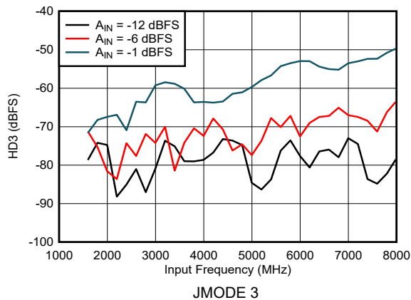
图 6-37. Dual Channel Mode: HD3 vs Input Frequency
