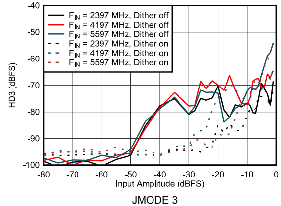
图 6-42. Dual Channel Mode: HD3 vs Input Amplitude
