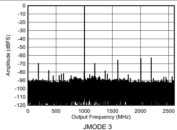
图 6-50. Dual Channel Mode: Single Tone Spectrum at 4197 MHz
