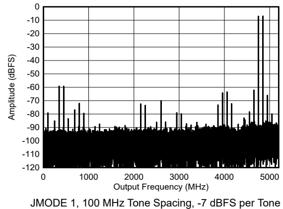
图 6-32. DES Mode: Two Tone Output Spectrum at 5597 MHz
