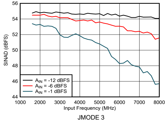
图 6-35. Dual Channel Mode: SINAD vs Input Frequency
