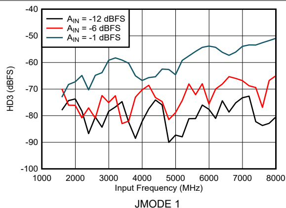
图 6-12. DES Mode: HD3 vs Input Frequency
