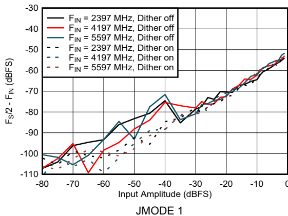
图 6-19. DES Mode: F_S/2 - F_{\text{IN}} vs Input Amplitude
