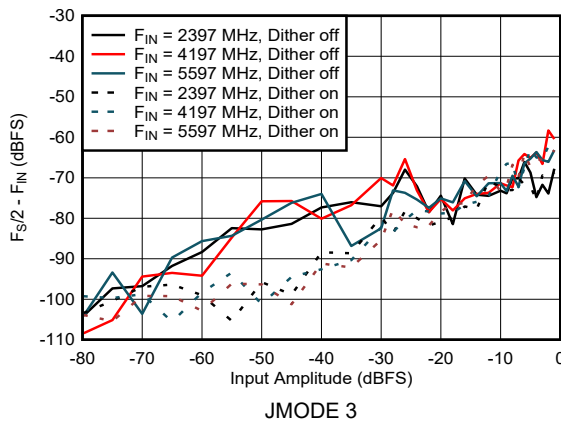
图 6-43. Dual Channel Mode: F_S/2 - F_{\text{IN}} vs Input Amplitude
