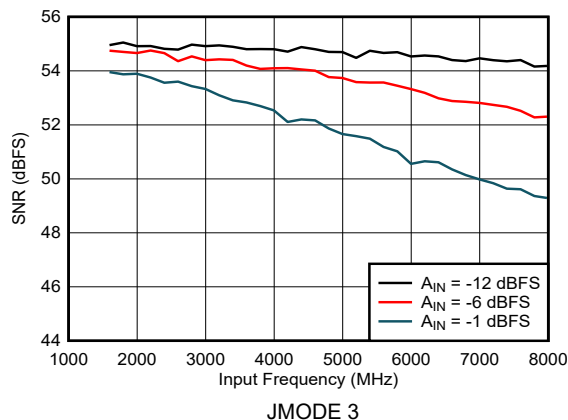
图 6-33. Dual Channel Mode: SNR vs Input Frequency
