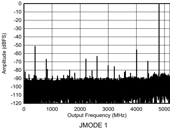
图 6-29. DES Mode: Single Tone Output Spectrum at 5597 MHz
