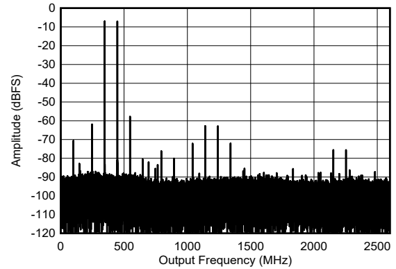
图 6-54. Dual Channel Mode: Dual Tone Spectrum at 5597 MHz
