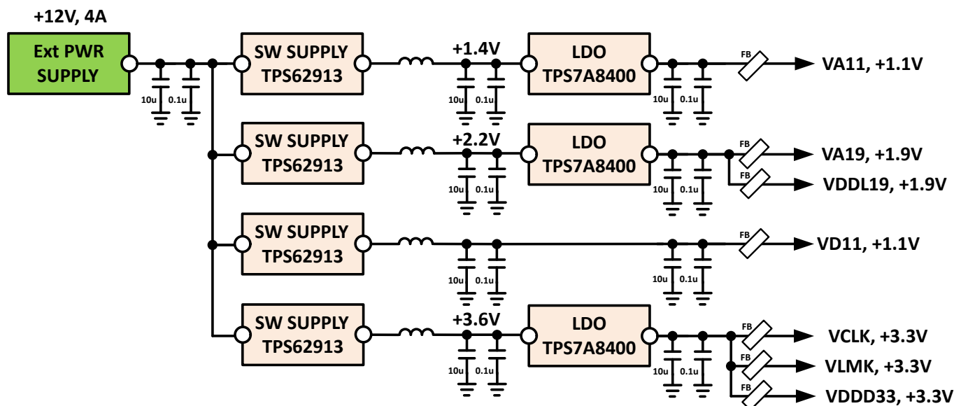
图 8-5. LDO Linear Regulator Approach Example
