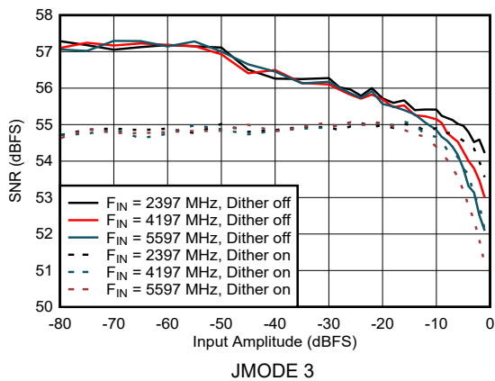
图 6-39. Dual Channel Mode: SNR vs Input Amplitude
