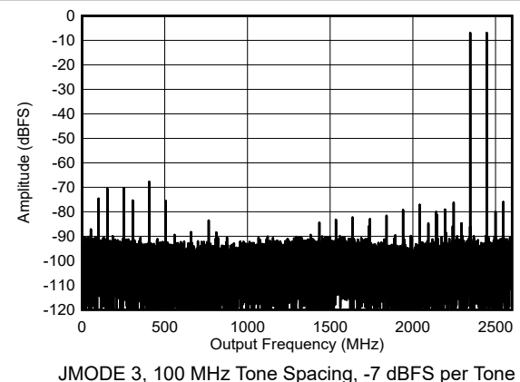
图 6-52. Dual Channel Mode: Dual Tone Spectrum at 2397 MHz
