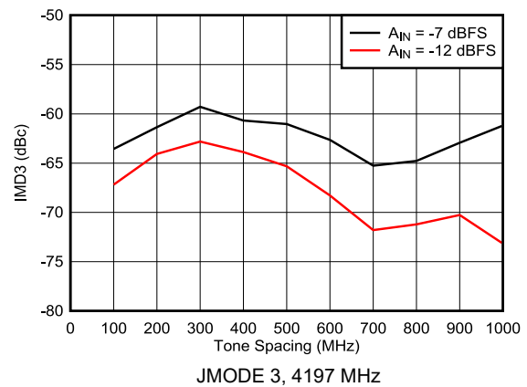
图 6-48. Dual Channel Mode: IMD3 vs Tone Spacing
