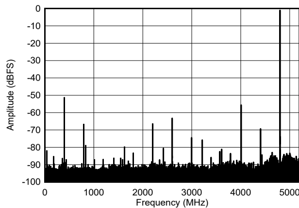
图 8-4. FFT for 5597 MHz Input Signal, 10.4 GSPS, JMODE1
