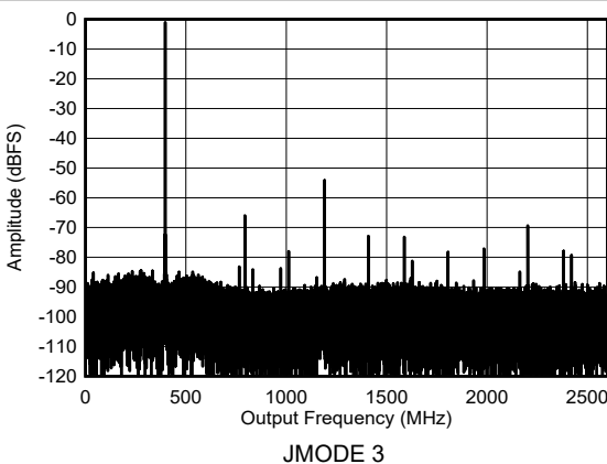
图 6-51. Dual Channel Mode: Single Tone Spectrum at 5597 MHz
