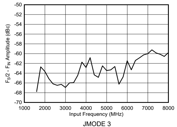
图 6-38. Dual Channel Mode: F_S/2 - F_{\text{IN}} vs Input Frequency
