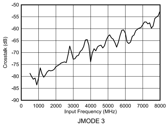
图 6-7. Dual Channel Mode: Crosstalk vs Input Frequency
