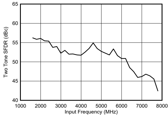
图 6-23. DES Mode: Two Tone SFDR vs Input Frequency
