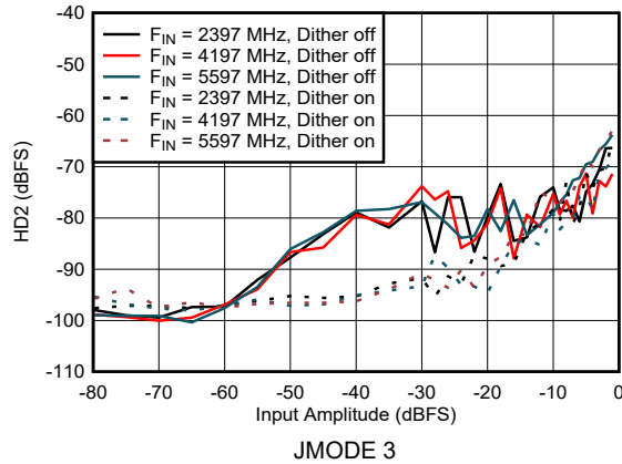
图 6-41. Dual Channel Mode: HD2 vs Input Amplitude
