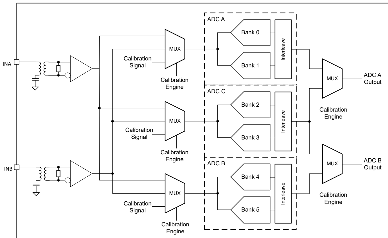
图 7-26. ADC12DJ5200SE Calibration System Block Diagram
