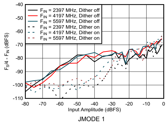
图 6-20. DES Mode: F_S/4 - F_{\text{IN}} vs Input Amplitude
