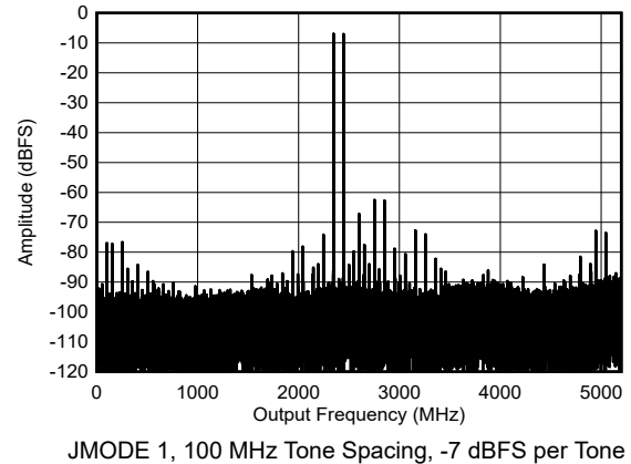
图 6-30. DES Mode: Two Tone Output Spectrum at 2397 MHz
