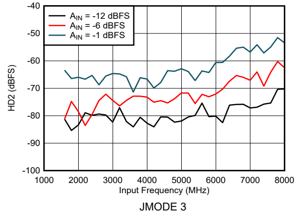
图 6-36. Dual Channel Mode: HD2 vs Input Frequency
