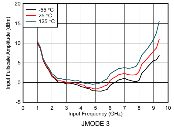
图 6-4. Dual Channel Mode: Input Fullscale vs Input Frequency
