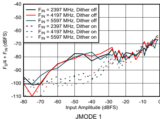
图 6-21. DES Mode: F_S/4 + F_{\text{IN}} vs Input Amplitude
