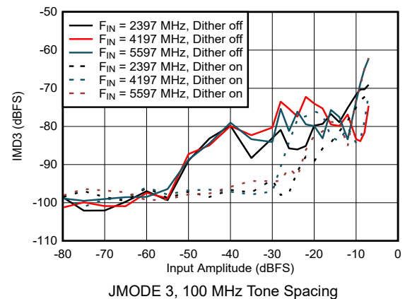
图 6-46. Dual Channel Mode: IMD3 vs Input Amplitude
