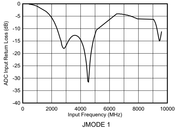
图 6-3. DES Mode: Input Return Loss vs Input Frequency
