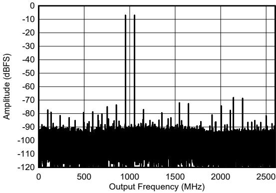
图 6-53. Dual Channel Mode: Dual Tone Spectrum at 4197 MHz
