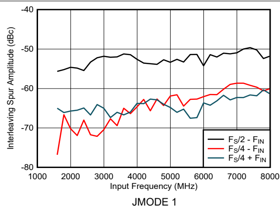
图 6-13. DES Mode: Interleaving Spurs vs Input Frequency
