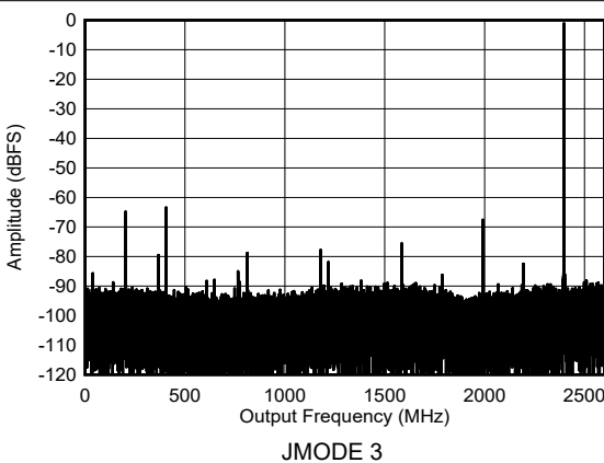
图 6-49. Dual Channel Mode: Single Tone Spectrum at 2397 MHz
