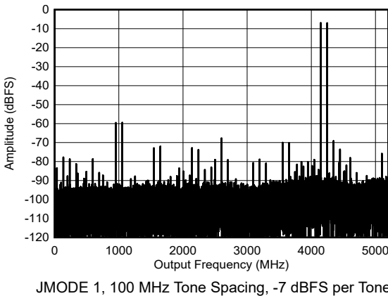
图 6-31. DES Mode: Two Tone Output Spectrum at 4197 MHz
