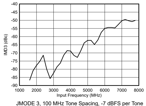
图 6-44. Dual Channel Mode: IMD3 vs Input Frequency
