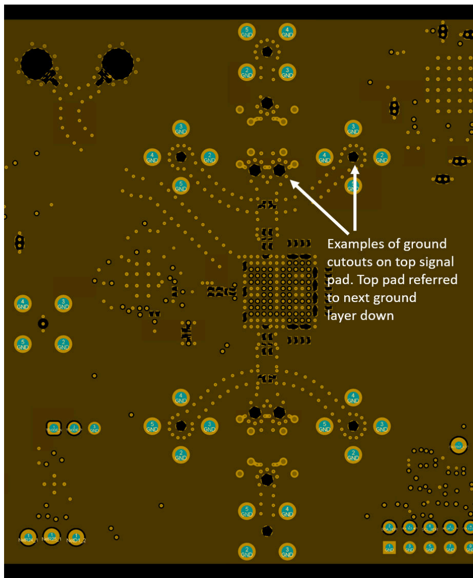
图 8-8. Example of Ground Cut-outs on Top Signal Pad
