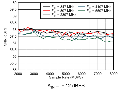
图 6-30. DES Mode: SNR vs Sample Rate and Input Frequency
