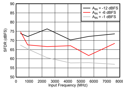
图 6-78. DES Mode: SFDR vs Input Frequency
