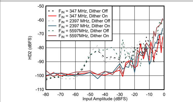
图 6-72. Dual Channel Mode: HD2 vs Input Amplitude and Dither
