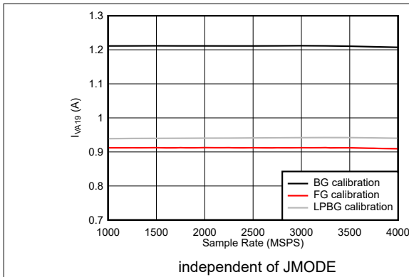
图 6-116. DES Mode: I_{VA19} vs Sample Rate
