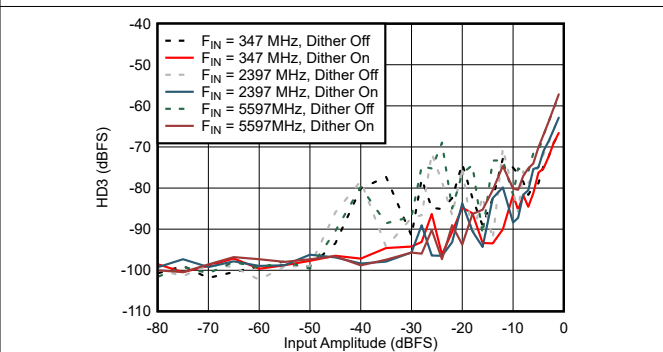
图 6-74. Dual Channel Mode: HD3 vs Input Amplitude and Dither
