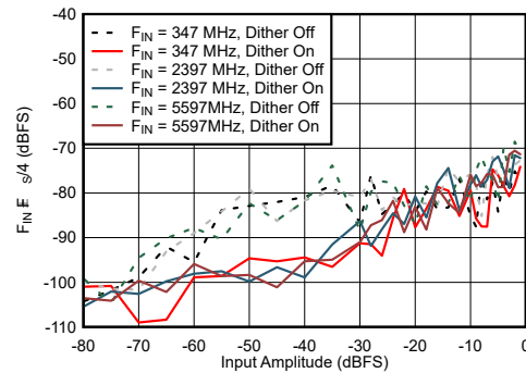
图 6-66. DES Mode: F_{\text{IN}} \pm F_S/4 vs Input Amplitude and Dither
