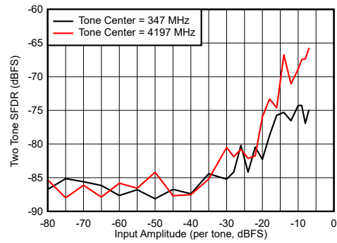
图 6-112. DES Mode: Two Tone SFDR vs Input Amplitude
