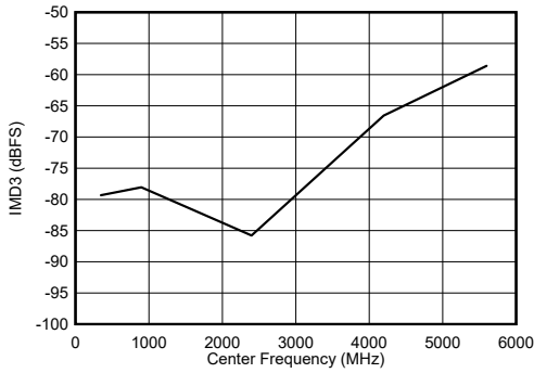
图 6-105. Dual Channel Mode: IMD3 vs Input Frequency
