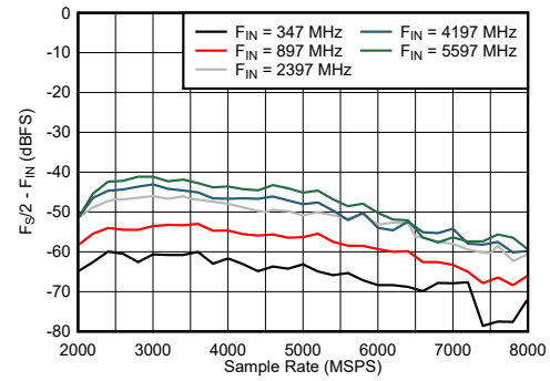
图 6-40. DES Mode: F_S/2 - F_{IN} vs Sample Rate and Input Frequency
