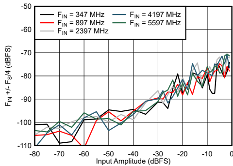
图 6-65. DES Mode: F_{\text{IN}} \pm F_S/4 vs Input Amplitude and Frequency
