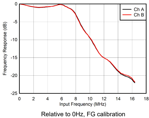
图 6-3. Dual Chanel Mode: Input Amplitude vs Input Frequency
