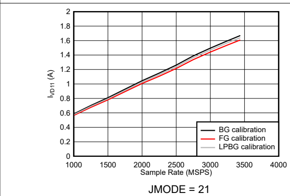
图 6-119. DES Mode: I_{VD11} vs Sample Rate
