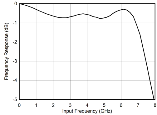
图 6-2. DES Mode: Input Response vs Input Frequency
