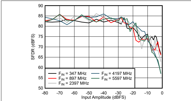
图 6-69. Dual Channel Mode: SFDR vs Input Amplitude and Frequency
