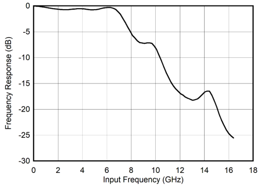
图 6-1. DES Mode: Input Amplitude vs Input Frequency
