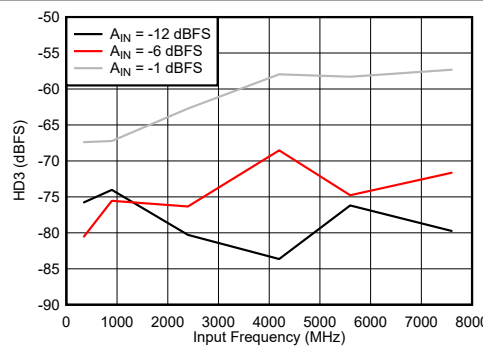
图 6-80. DES Mode: HD3 vs Input Frequency
