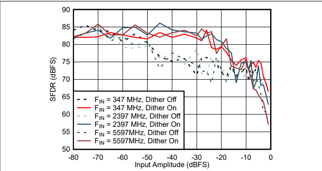
图 6-70. Dual Channel Mode: SFDR vs Input Amplitude and Dither
