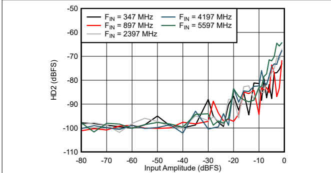
图 6-59. DES Mode: HD2 vs Input Amplitude and Frequency
