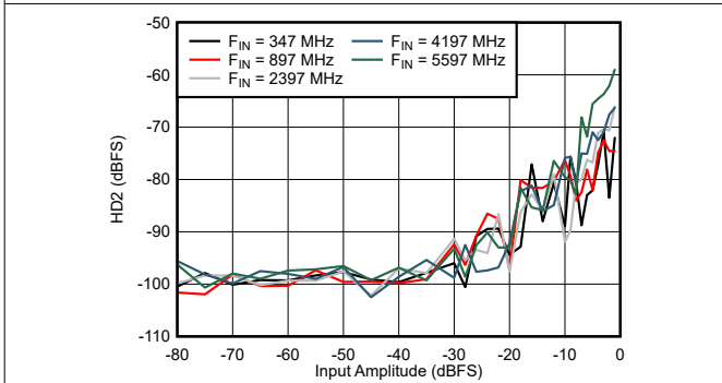
图 6-71. Dual Channel Mode: HD2 vs Input Amplitude and Frequency
