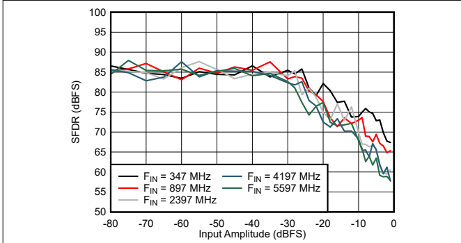
图 6-57. DES Mode: SFDR vs Input Amplitude and Frequency
