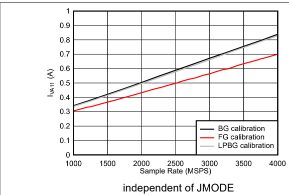
图 6-117. DES Mode: I_{VA11} vs Sample Rate
