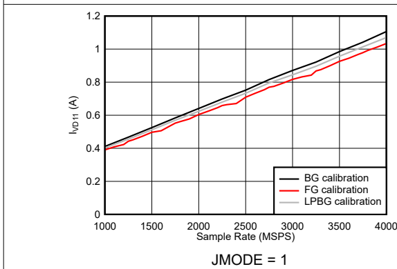
图 6-118. DES Mode: I_{VD11} vs Sample Rate
