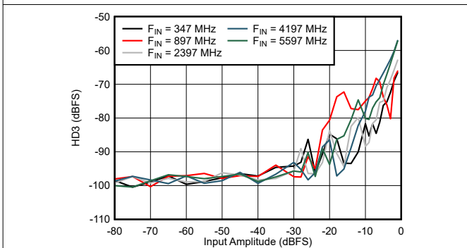
图 6-73. Dual Channel Mode: HD3 vs Input Amplitude and Frequency
