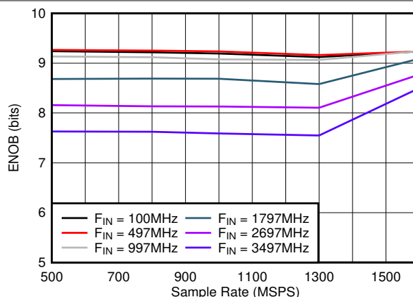
图 6-26. ENOB vs Sample Rate
