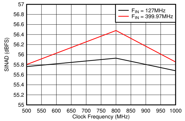
图 6-30. SINAD vs Sample Rate
