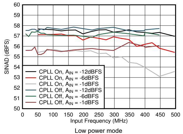
图 6-56. SINAD vs A_{IN} and C-PLL
