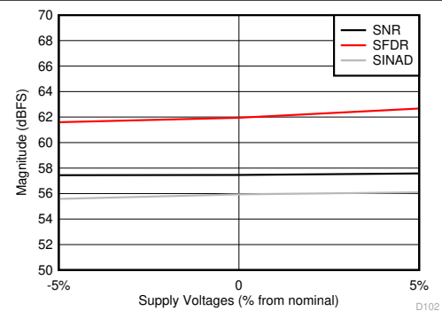
图 6-62. SNR, SFDR and SINAD vs Supply Voltages All supplies changed together, low power mode, F_S = 1000 MSPS
