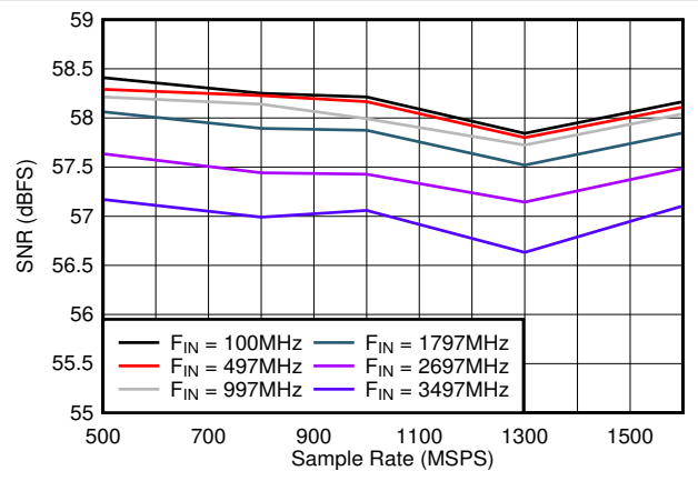
图 6-24. SNR vs Sample Rate
