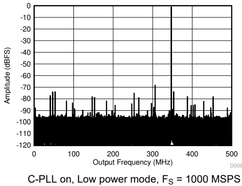
图 6-13. Single Tone FFT at 347 MHz and -1 dBFS
