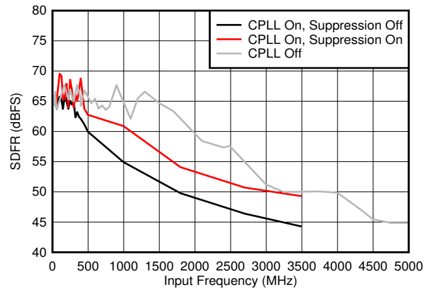
图 6-40. SFDR vs F_{IN} and C-PLL modes
