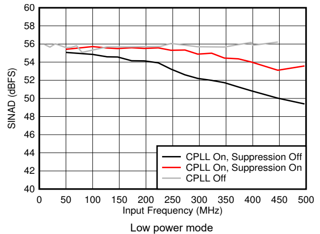
图 6-46. SINAD vs F_{IN} and C-PLL modes
