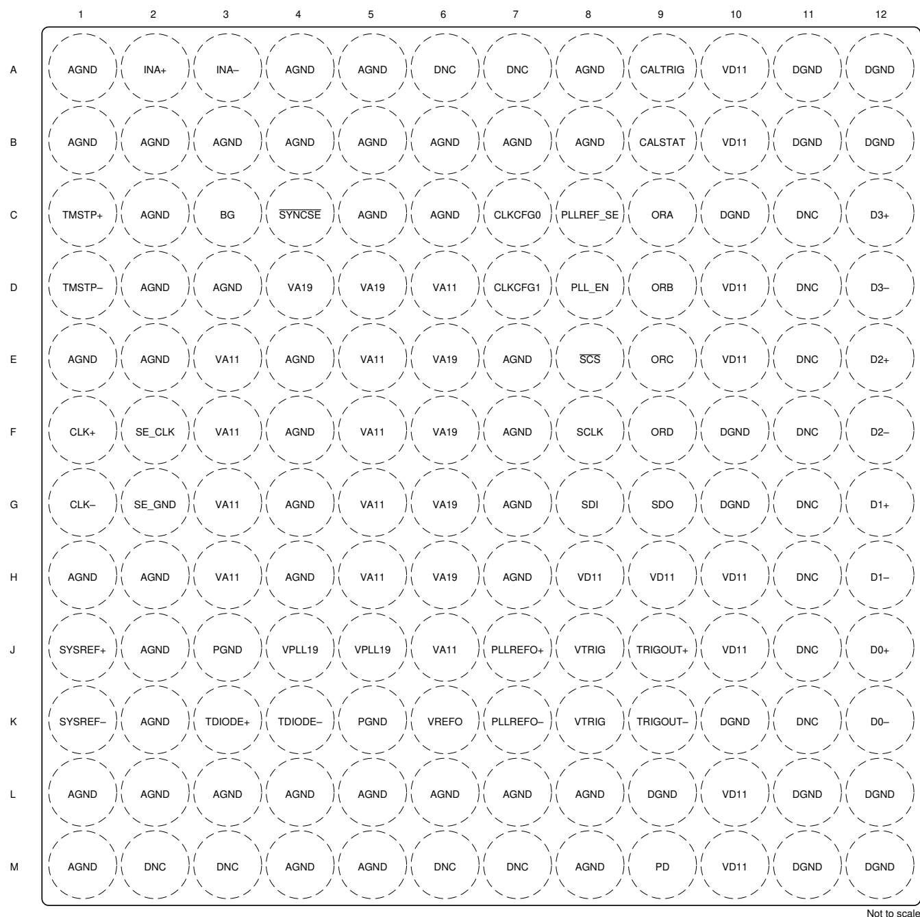
图 5-3. Single Channel AAV Package, 144-Ball Flip Chip BGA (Top View)
