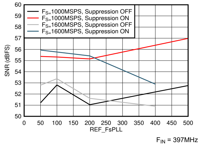
图 6-38. SNR vs F_{REF} and Suppression
