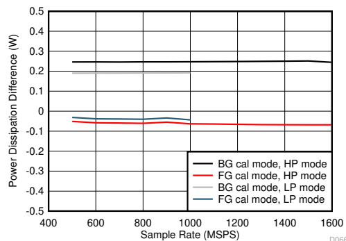
Difference to lower power background calibration, JMODE independent 图 6-110. Dual Channel, Power Dissipation Change with Calibration Mode
