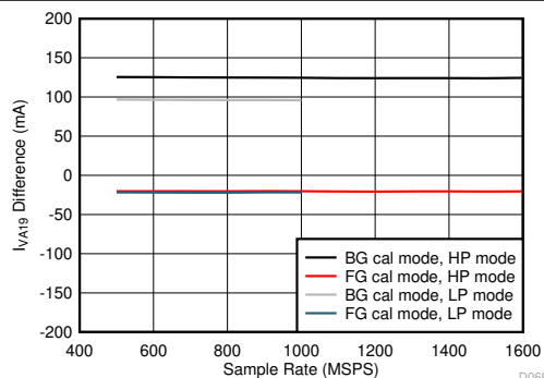
Difference to lower power background calibration, JMODE independent 图 6-112. Quad Channel, I_{VA19} Change with Calibration Mode
