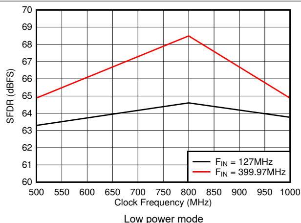
图 6-27. SFDR vs Sample Rate
