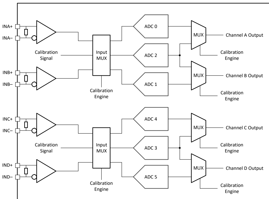
图 7-15. Quad Channel Calibration System Block Diagram
