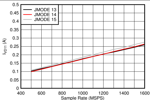
Low power background calibration mode 图 6-108. Single Channel, I_{VD11} vs F_S and JMODE 13 - 15
