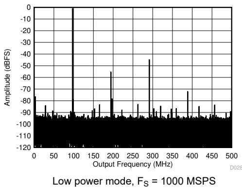
图 6-15. Single Tone FFT at 2097 MHz and -1 dBFS
