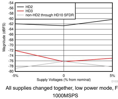
图 6-63. HD2, HD3 and Worst non-HD Spur vs Supply Voltage
