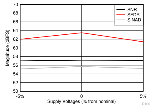
图 6-60. SNR, SFDR and SINAD vs Supply Voltage All supplies changed together, high power mode
