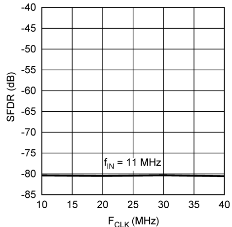
Figure 31. SFDR vs. f_{CLK}
