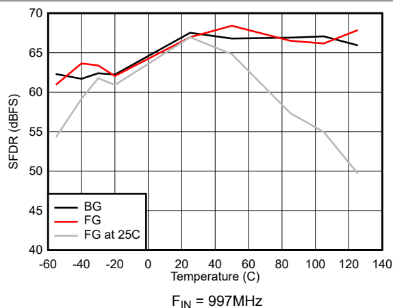
图 7-35. SFDR vs Temperature
