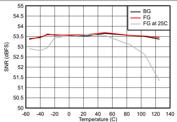
图 7-34. SNR vs Temperature
