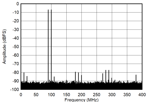
图 7-50. Dual Tone FFT at 95 MHz
