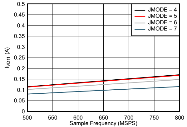
图 7-98. Single Channel, I_{VD11} vs F_S for JMODES 4 - 7
