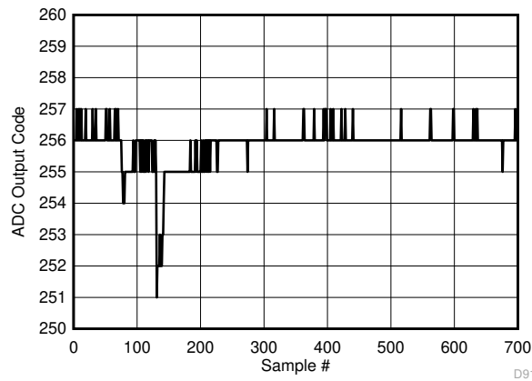
图 7-129. Background Calibration Core Transition (DC Signal)
