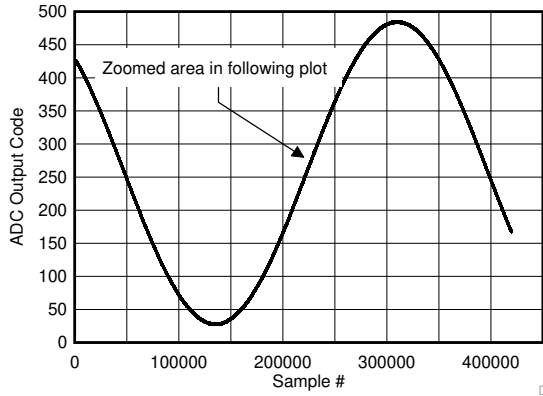
图 7-127. Background Calibration Core Transition (AC Signal)
