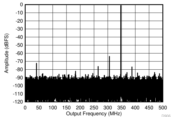
F_S = 1000\text{MSPS} , Low Power Mode 图 7-12. Single Tone FFT at 347 MHz and -1 dBFS
