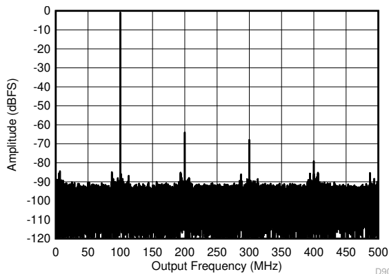
F_S = 1000\text{MSPS} , Low Power Mode 图 7-11. Single Tone FFT at 99.997 MHz and -1 dBFS
