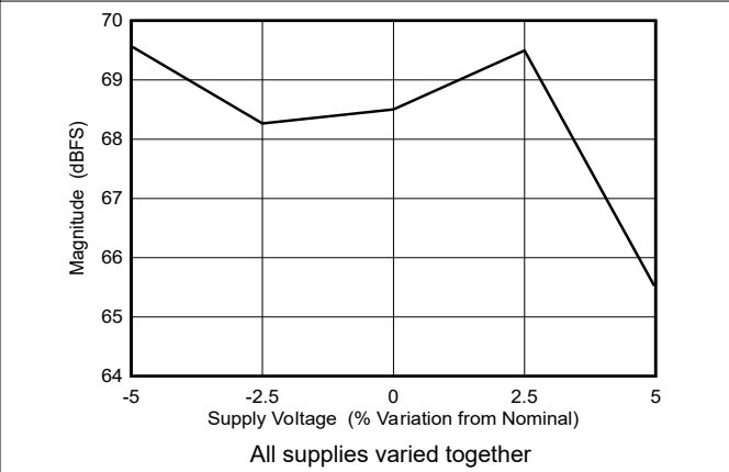
图 5-96. Dual Channel Mode: SFDR vs Supply Voltage
