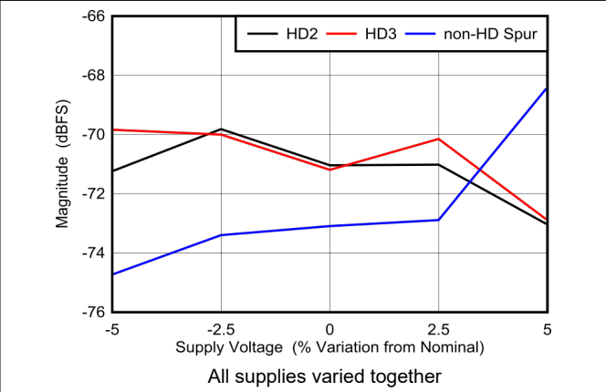
图 5-94. DES Mode: HD2, HD3 and Worst Spur vs Supply Voltage
