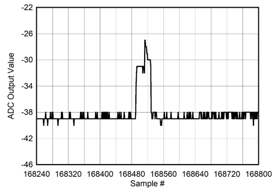
图 5-120. Background Calibration Core Transition (AC Signal Zoomed)
