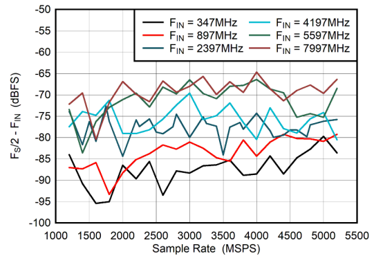
图 5-56. Dual Channel Mode: F_s/2 - F_{IN} vs Sample Rate
