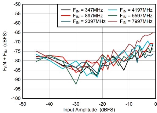
图 5-67. DES Mode: F_S/4 + F_{IN} vs Input Amplitude
