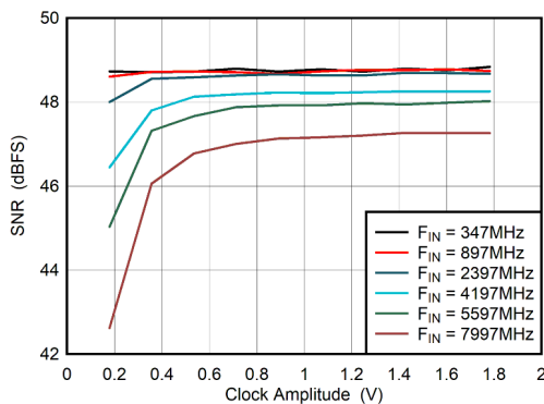
图 5-83. Dual Channel Mode: SNR vs Clock Amplitude
