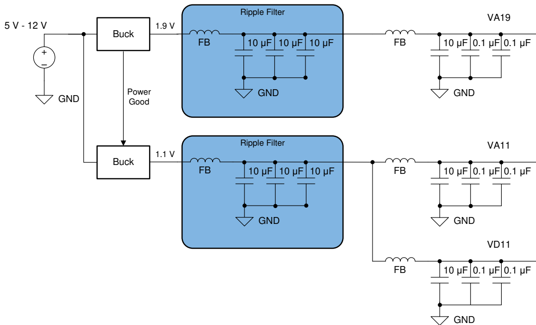
图 7-2. LDO Linear Regulator Approach Example
