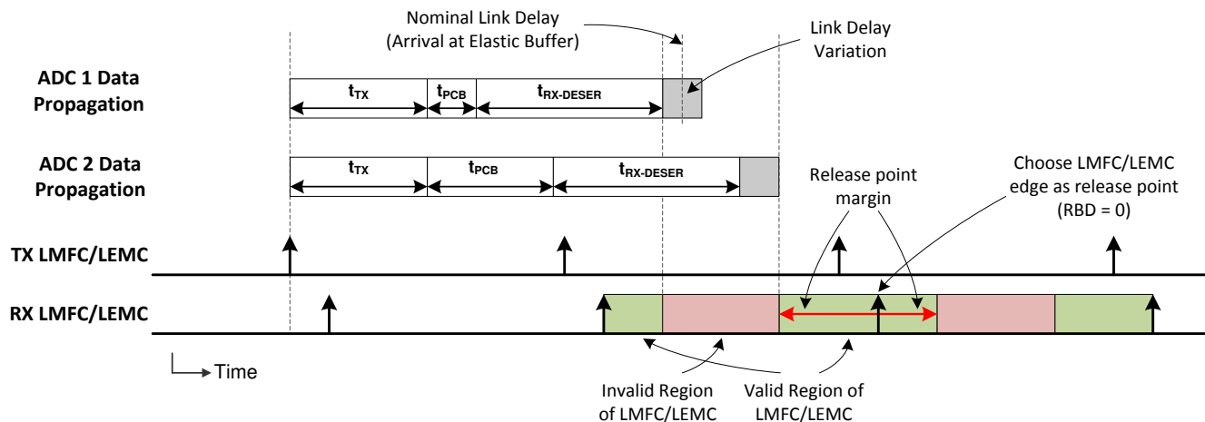
图 6-12. LMFC/LEMFC Valid Region Definition for Elastic Buffer Release Point Selection
