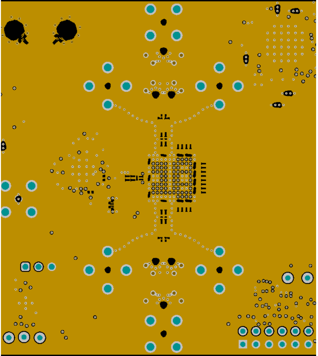
图 7-5. GND1 Cutouts to Optimize Impedance of Component Pads
