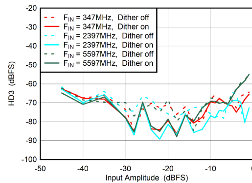
图 5-78. Dual Channel Mode: HD3 vs Input Amplitude and Dither
