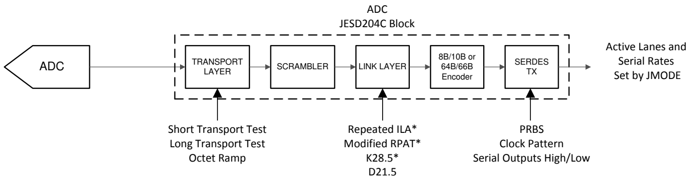
图 6-13. Test Mode Insertion Points
