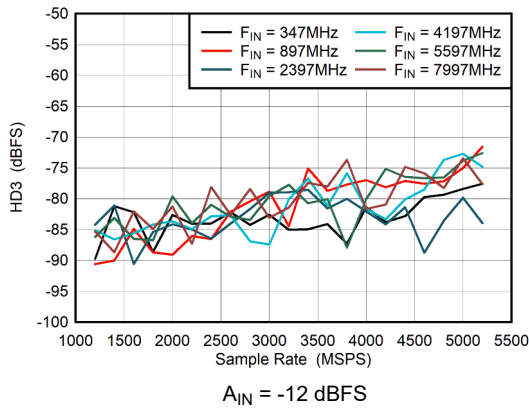
图 5-55. Dual Channel Mode: HD3 vs Sample Rate
