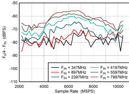
图 5-43. DES Mode: F_S/4 - F_{IN} vs Sample Rate
