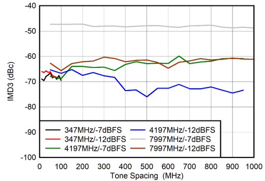
图 5-102. DES Mode: IMD3 vs Tone Spacing
