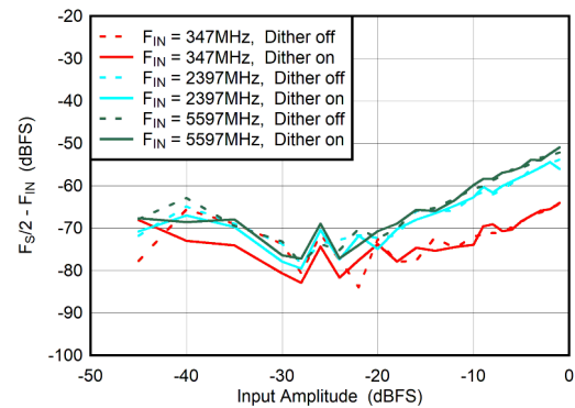
图 5-66. DES Mode: F_S/2 - F_{IN} vs Input Amplitude and Dither
