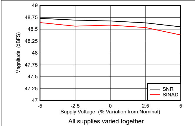
图 5-95. Dual Channel Mode: SNR and SINAD vs Supply Voltage
