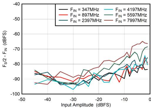
图 5-79. Dual Channel Mode: F_{S/2} - F_{IN} vs Input Amplitude
