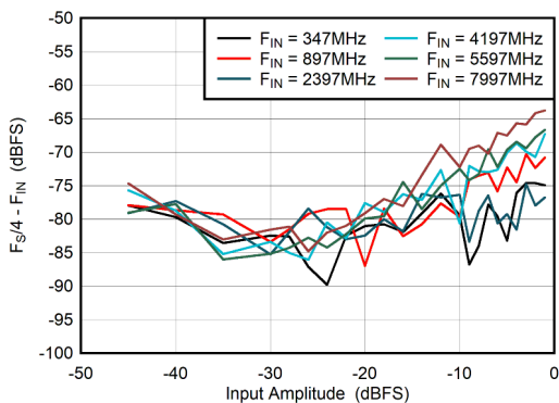
图 5-69. DES Mode: F_S/4 - F_{IN} vs Input Amplitude
