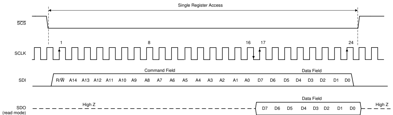
图 6-15. Serial Interface Protocol: Single Read/Write
