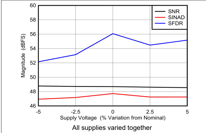
图 5-93. DES Mode: SNR, SINAD and SFDR vs Supply Voltage
