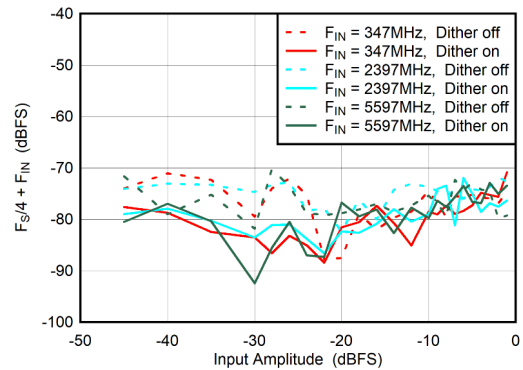
图 5-68. DES Mode: F_S/4 + F_{IN} vs Input Amplitude and Dither
