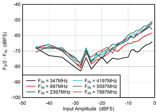
图 5-65. DES Mode: F_S/2 - F_{IN} vs Input Amplitude
