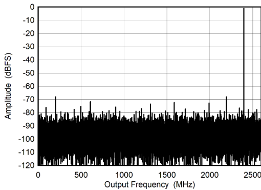
图 5-19. Dual Channel Mode: Single Tone FFT at 2397 MHz
