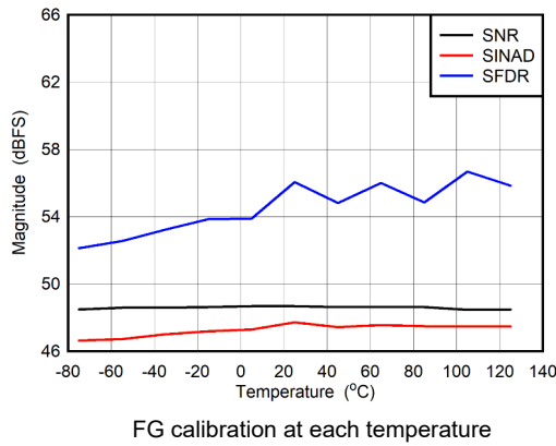
图 5-85. DES Mode: SNR, SINAD and SFDR vs Temperature
