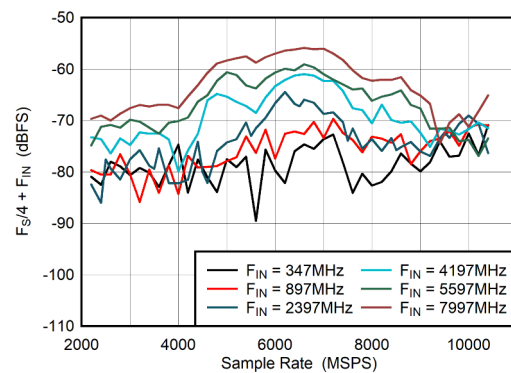
图 5-42. DES Mode: F_S/4 + F_{IN} vs Sample Rate
