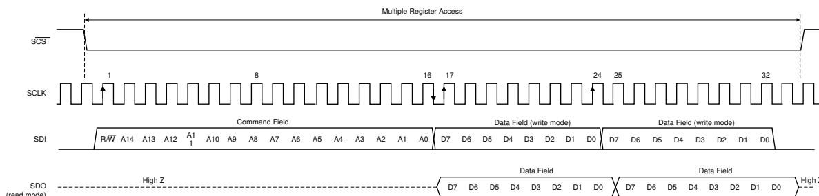
图 6-16. Serial Interface Protocol: Streaming Read/Write
