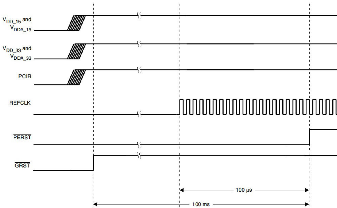
图 6-1. Power-Up Sequence
