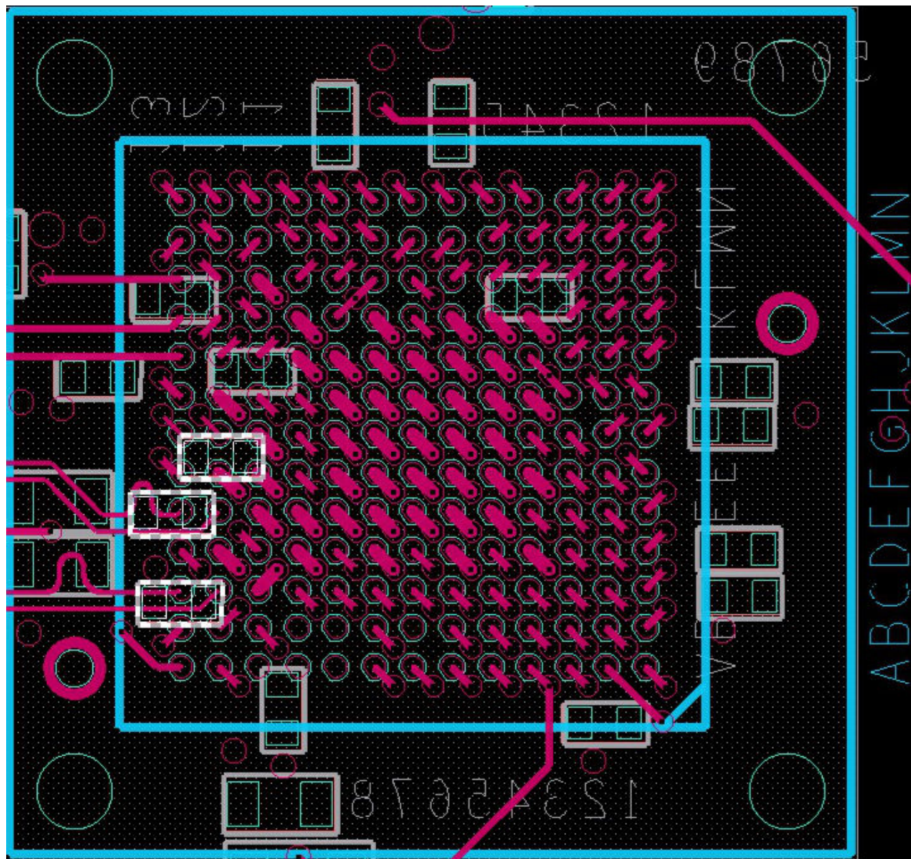
图 9-9. BGA Via Routing Layout
