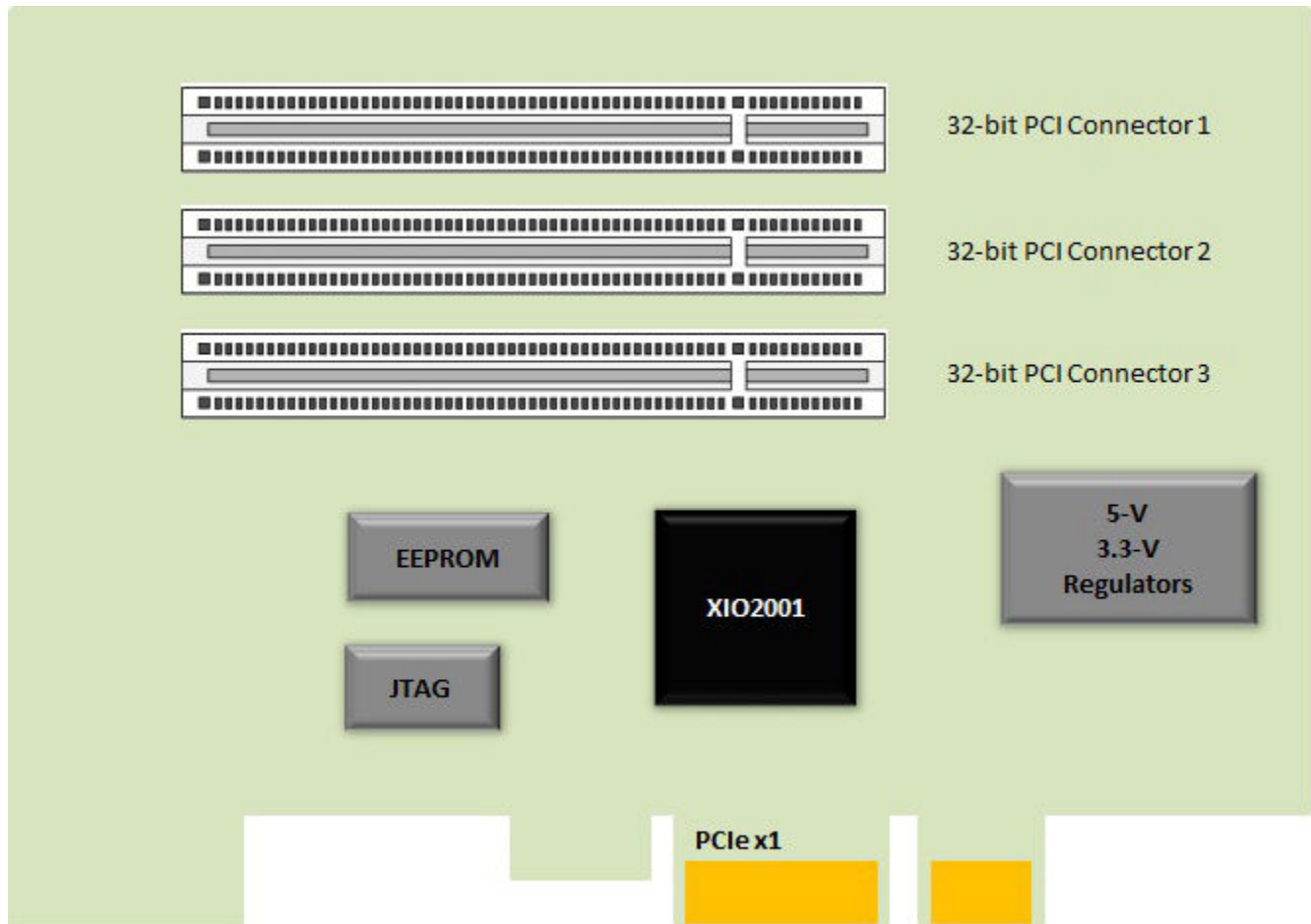
图 9-1. Typical Application
