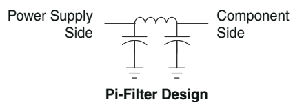
图 9-12. Filter Designs
