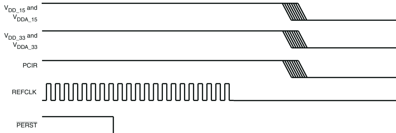
图 6-2. Power-Down Sequence
