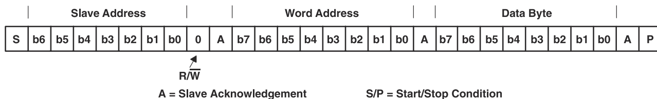
图 8-12. Serial-Bus Protocol - Byte Write
