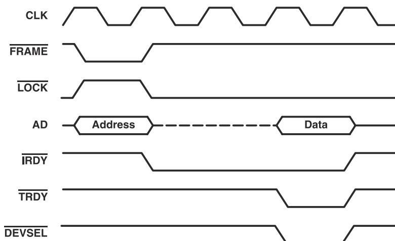
图 8-7. Continuing a Locked Sequence
