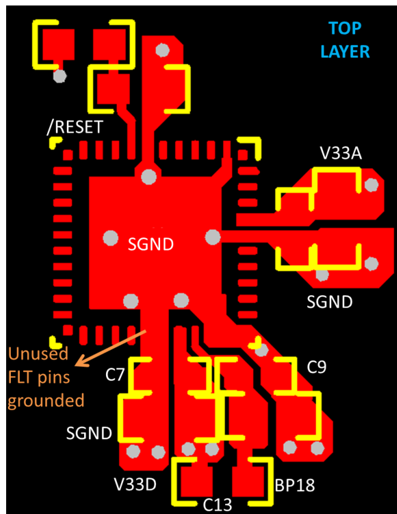
图 12-11. UCD3138 and UCD3138064 40 Pin Layout Top Layer
