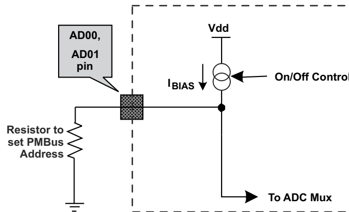
图 9-17. PMBUS Address Detection Method
