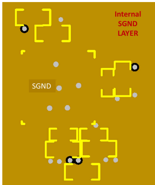
图 12-12. UCD3138 and UCD3138064 40 Pin Layout Internal SGND Layer
