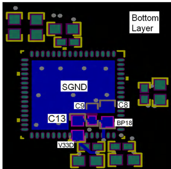
图 12-17. Alternative 64 Pin UCD3138 and UCD3138064 Layout Bottom Layer
