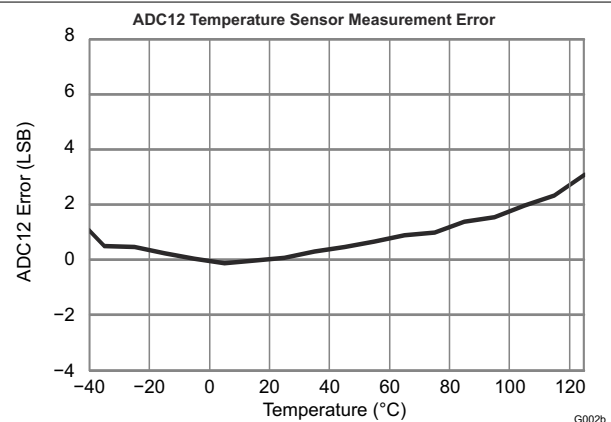
图 8-8. ADC12 Temperature Sensor Measurement Error vs Temperature
