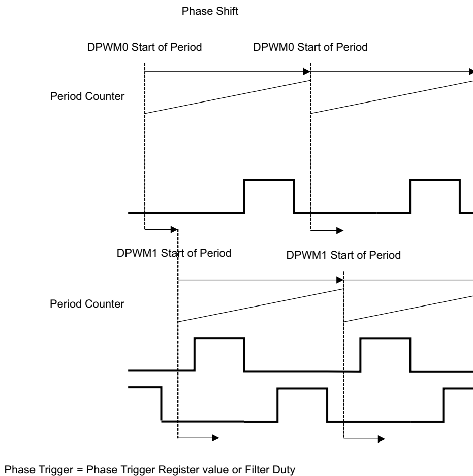
图 9-23. Phase Shifting
