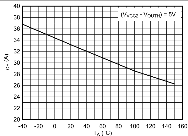
图 6-1. I_{O_{UH}} vs. Temperature
