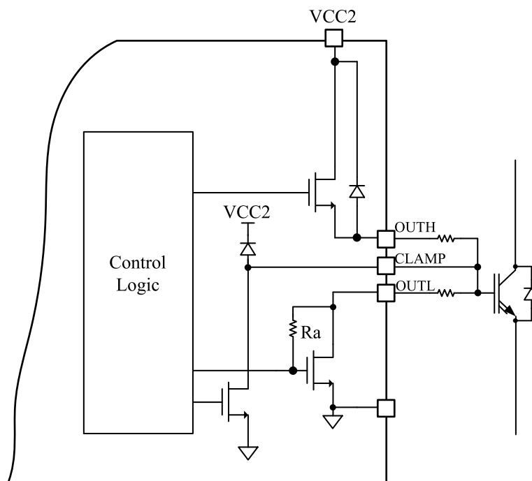
图 7-12. CLAMP, OUTH, and OUTL Clamping Circuits
