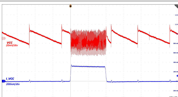
图 8-5. 负载瞬态 : VINP = 5.0V , VCC = 3.3V , C OUT2 = 22 μF , I VCC = 0mA - 300mA - 0mA
