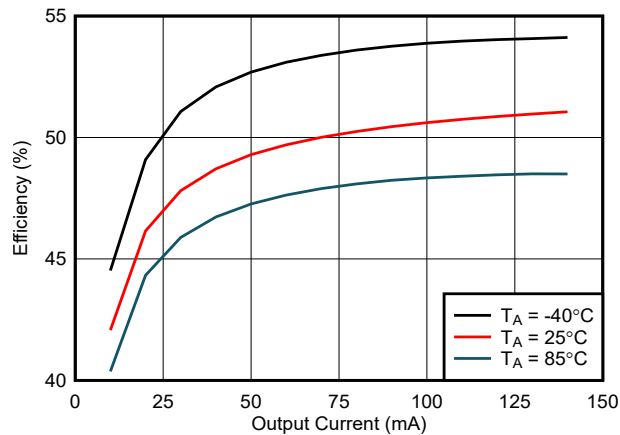
图 6-13. 效率与负载电流 ( I_{VCC} ) 间的关系: V_{CC} = 5.0\text{V} , V_{INP} = 3.3\text{V} , C_{OUT2} = 22\text{ }\mu\text{F}
