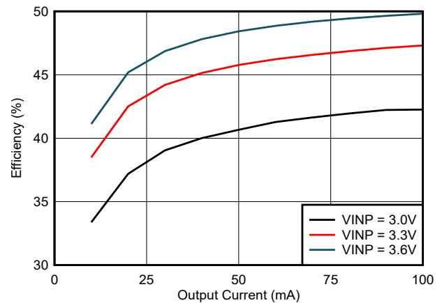
图 6-14. 效率与负载电流 ( I_{VCC} ) 间的关系: V_{CC} = 5.5\text{V} , T_A = 25^\circ\text{C} , C_{OUT2} = 22\text{ }\mu\text{F}
