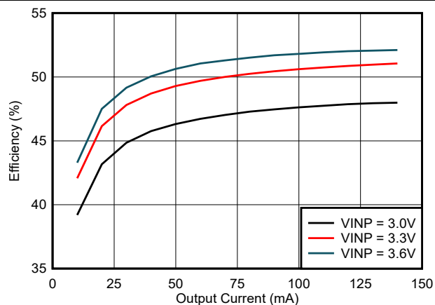
图 6-12. 效率与负载电流 ( I_{VCC} ) 间的关系：VCC = 5.0V, T_A = 25°C, COUT2 = 22 μF
