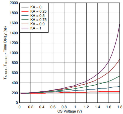
图 6-6. Delay Time T_{AFSET} and T_{BESET} (Over CS Voltage and Selected K_{EF} for R_{EF} Equal 90k \Omega )
