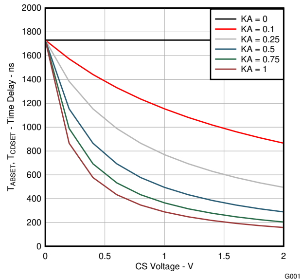
图 6-3. Delay Time set T_{ABSET} and T_{CDSET} (Over CS Voltage Variation and Selected K_A for R_{AB} and R_{CD} Equal 90 k \Omega )
