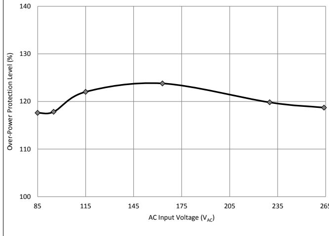
图 52. OPP Level in Universal AC Line
