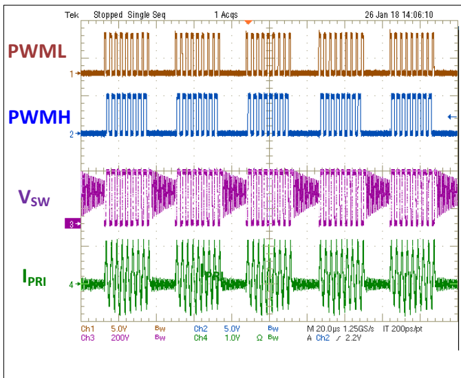
图 48. ABM Waveforms at V_{IN} = 115 V_{RMS} and I_O = 0.9 A
