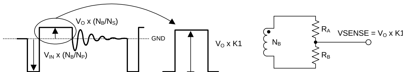
Figure 22. V_{OUT} Sense Using the Positive Swing on the Sense Winding
