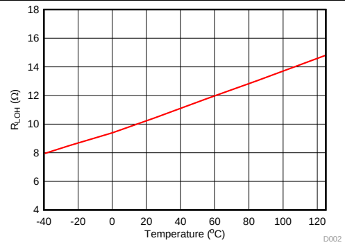
图 21. LO Output Pull-Up Resistance vs Temperature
