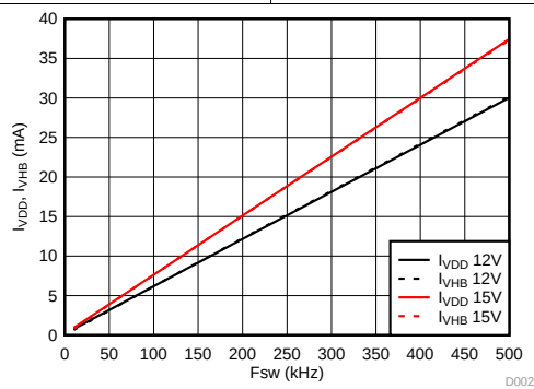
图 26. VDD 和 HB Operating Current with No Load vs Switching Frequency
