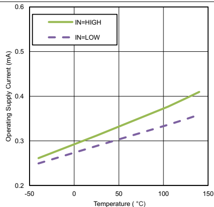
图 22. Operating Supply Current vs. Temperature (Output In DC On/Off Condition)
