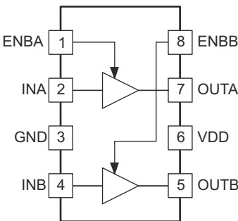
图 5-2. UCC27424-Q1: D or DGN Package 8-Pin SOIC or MSOP With PowerPAD Dual Noninverting, Top View
