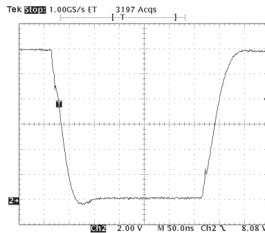
图 7-2. Pulse Response
