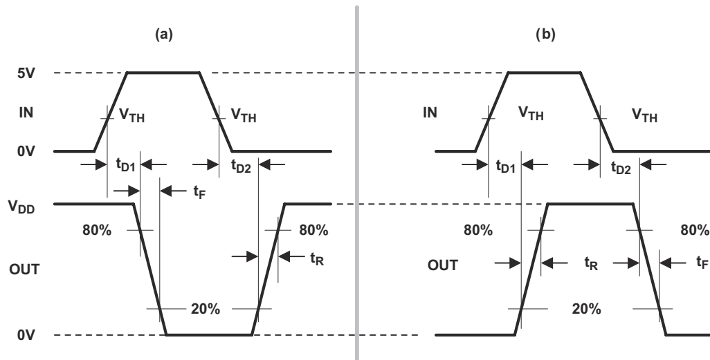
图 7-1. Switching Waveforms for (a) Inverting Input to (b) Output Times
