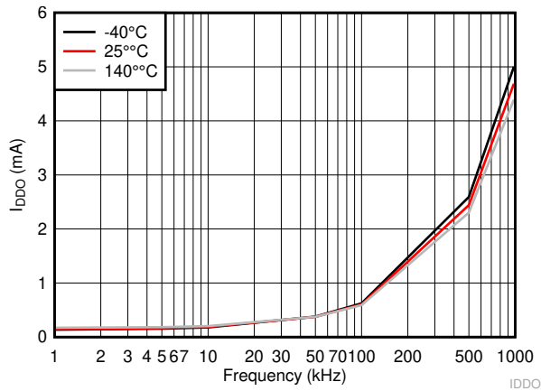
A. C_L = 0\text{ F} V_{DD} = V_{HB} = 12\text{ V}
