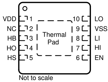
图 5-1. DRC Package 10-Pin VSON With Exposed Thermal Pad (Top View)
