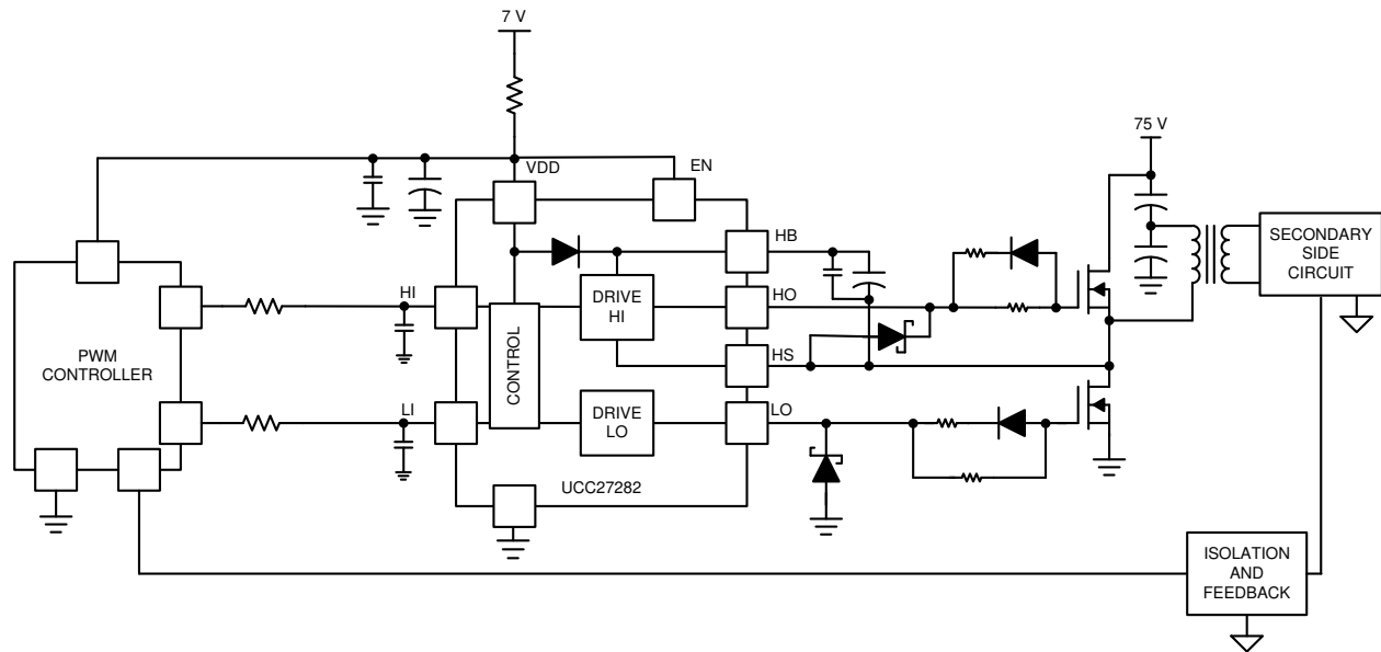
图 8-1. Typical Application
