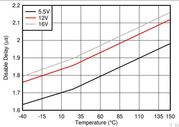
图 6-13. Disable Delay
