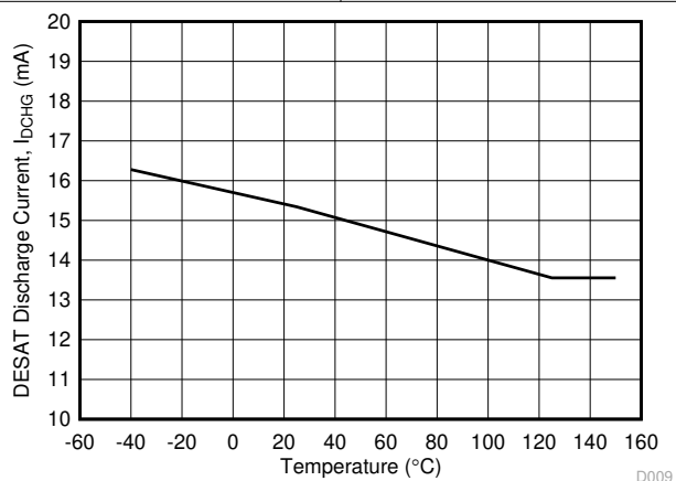
图 6-30. I_{\text{DCHG}} DESAT Discharge Current vs Temperature
