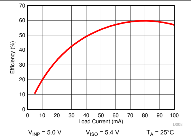
图 6-13. Power Supply Efficiency vs Load Current ( I_{ISO} )
