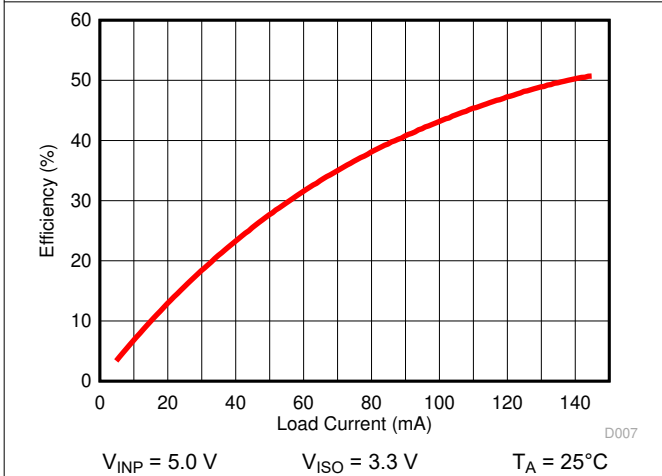
图 6-14. Power Supply Efficiency vs Load Current ( I_{ISO} )
