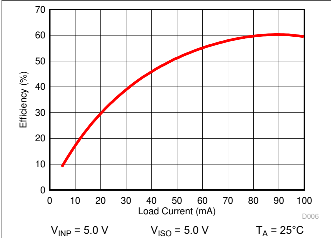
图 6-12. Power Supply Efficiency vs Load Current ( I_{ISO} )
