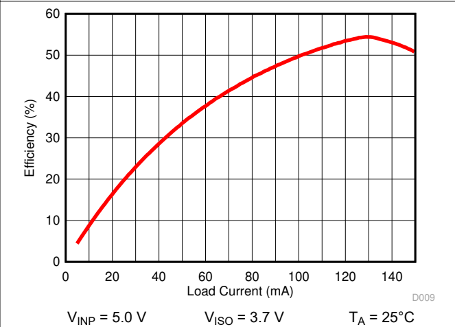
图 6-15. Power Supply Efficiency vs Load Current ( I_{ISO} )
