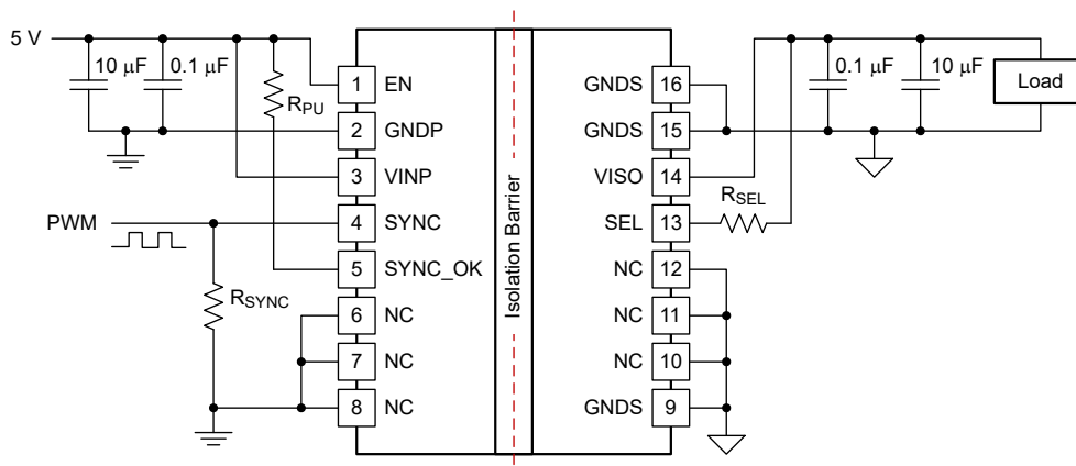
图 8-1. Typical Application
