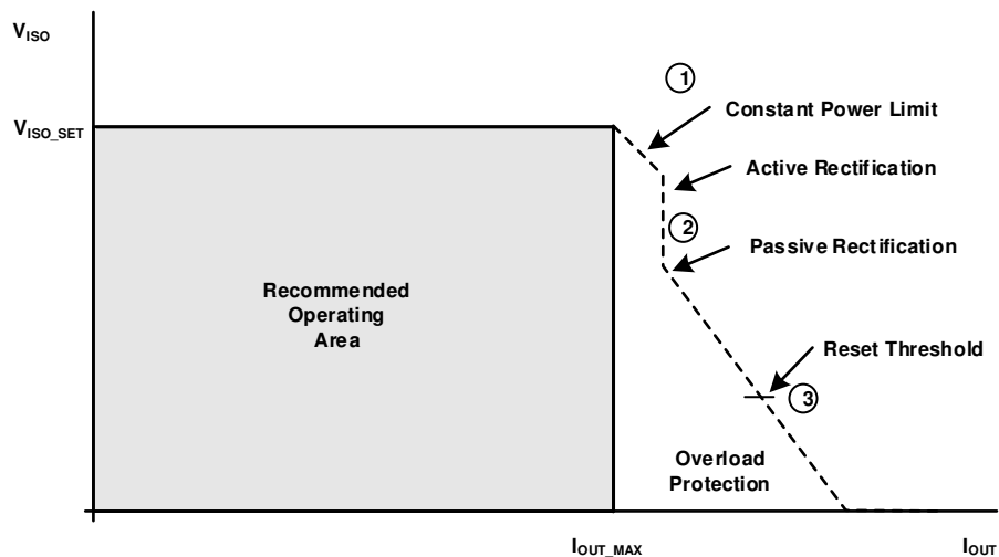
图 7-1. V_{ISO} Load Recommended Operating Area Description
