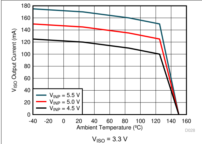
图 6-10. Maximum V_{ISO} Output Current vs. Temperature
