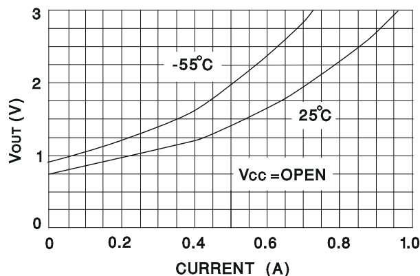
图 7-3. Output Voltage vs Output Current
