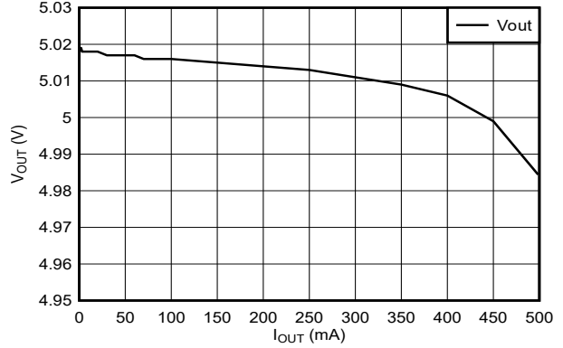
图 5-2. Load Regulation at T_J = 25^\circ\text{C} (New Chip)
