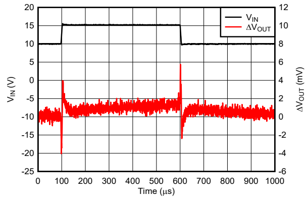
图 7-5. V_{IN} vs V_{OUT} at T_J = 25^\circ\text{C} (New Chip)
