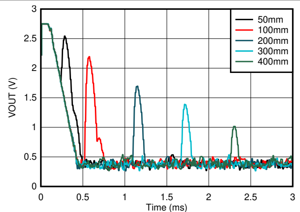
图 8-7. TUSS4470 400 kHz Ranging at 20-V Driver
