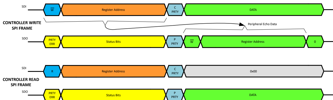
图 7-10. SPI Transfer Sequence
