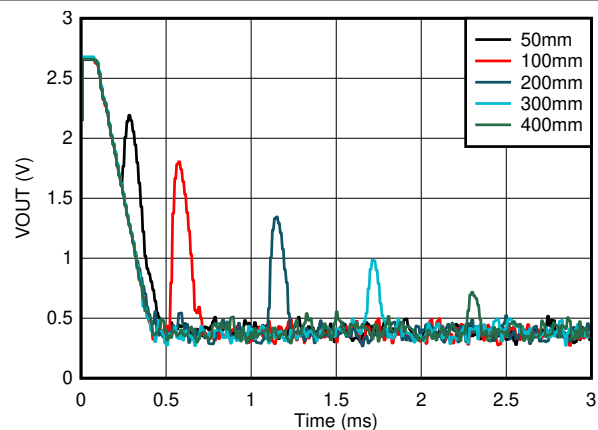
图 8-6. TUSS4470 400 kHz Ranging at 5-V Drive
