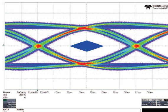
Figure 47. Downstream Port 1
