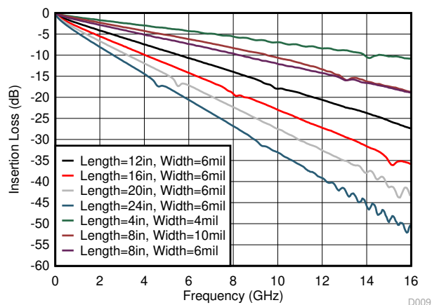
图 9-5. Insertion Loss of FR4 PCB Traces
