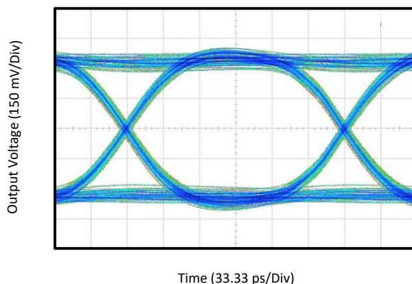
图 6-10. USB 3.1 Gen1 Eye-Pattern Performance with 12-inch Input PCB Trace at 5 Gbps
